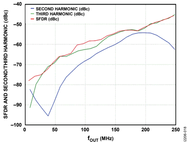
Figure 13. SFDR, 2 nd and 3 rd Harmonics vs. f_{OUT} , Maximum I_{OUTFS} (DAC Gain)
