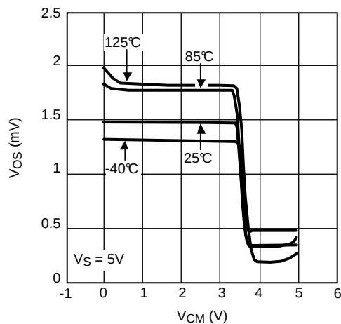
Figure 4. V_{OS} vs V_{CM} (Unit 3)
