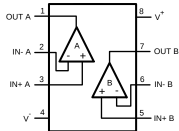
D Package 8-Pin SOIC Top View
