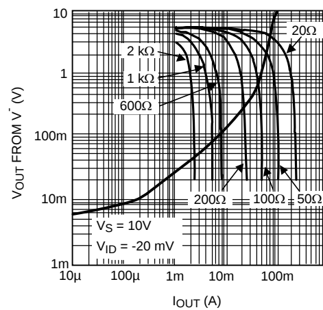
Figure 48. Steady-State Output Sinking Characteristics With Load Lines
