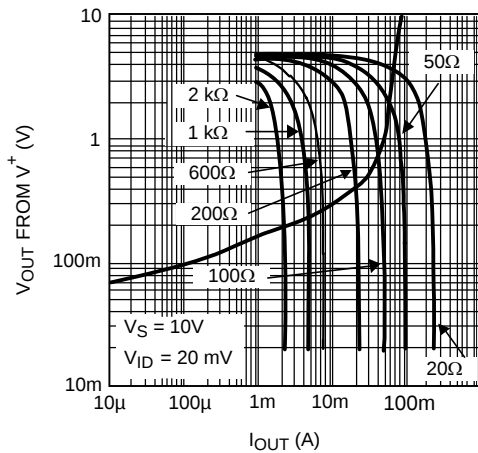
Figure 47. Steady-State Output Sourcing Characteristics With Load Lines
