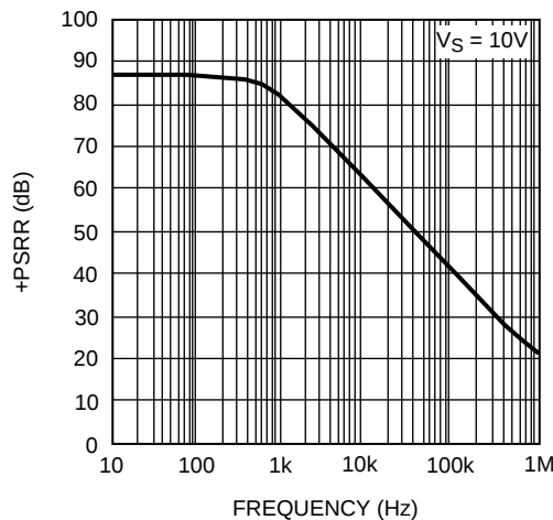
Figure 35. +PSRR vs Frequency
