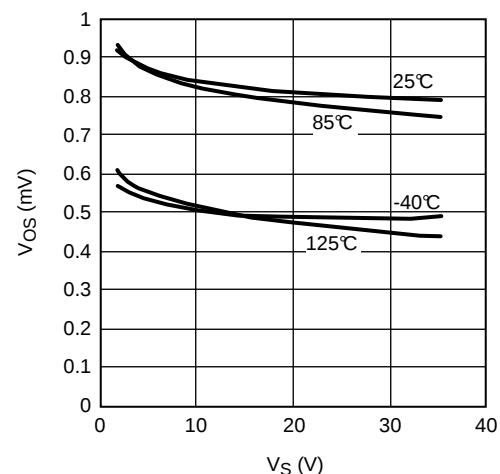
Figure 10. V_{OS} vs V_S (Unit 3)
