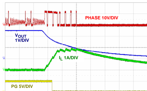
FIGURE 18. OUTPUT SHORT CIRCUIT (5µs/DIV)
