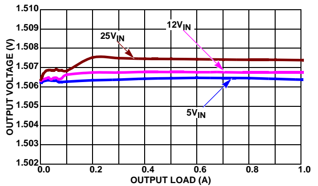
FIGURE 7. V_{OUT} REGULATION vs LOAD, 500kHz, 1.5\text{V}_{OUT}
