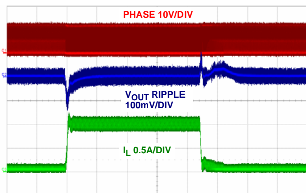
FIGURE 14. LOAD TRANSIENT (200µs/DIV)
