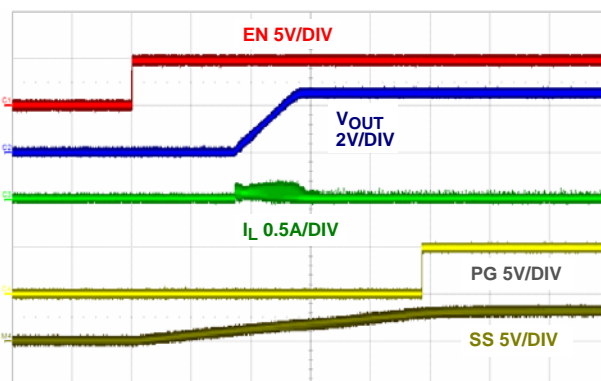
FIGURE 15. SOFT-START AT NO LOAD (2ms/DIV)
