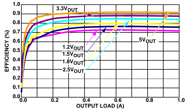
FIGURE 3. EFFICIENCY vs LOAD, 500kHz, 12\text{V}_{IN}
