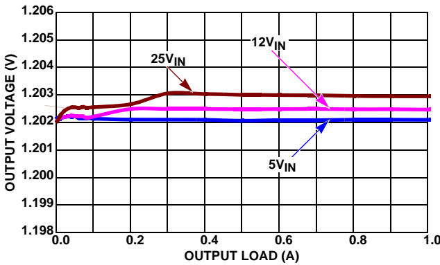
FIGURE 6. V_{OUT} REGULATION vs LOAD, 500kHz, 1.2\text{V}_{OUT}
