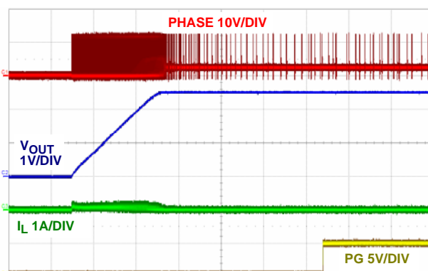
FIGURE 19. OUTPUT SHORT CIRCUIT RECOVERY (1ms/DIV)
