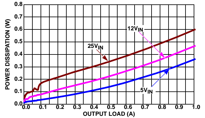
FIGURE 5. POWER DISSIPATION vs LOAD, 500kHz, 2.5\text{V}_{OUT}
