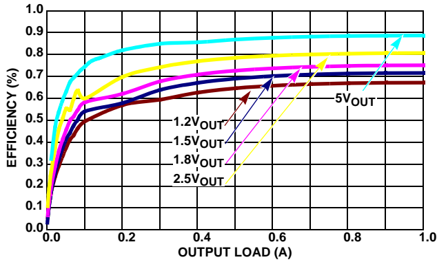
FIGURE 4. EFFICIENCY vs LOAD, 500kHz, 25\text{V}_{IN}
