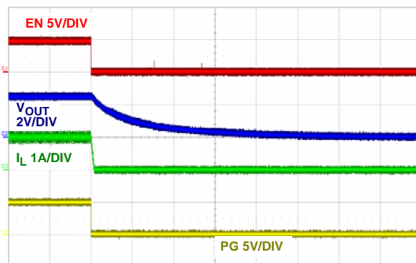
FIGURE 17. SHUT DOWN CIRCUIT (100µs/DIV)
