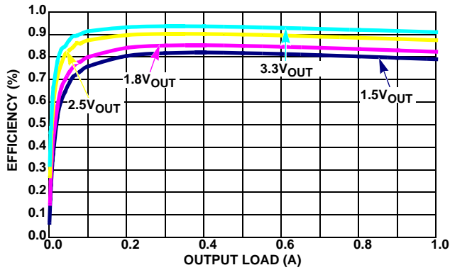
FIGURE 2. EFFICIENCY vs LOAD, 500kHz, 5\text{V}_{IN}
