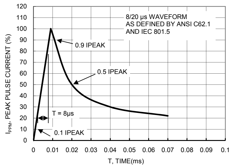
FIG. 8 PULSE WAVEFORM
