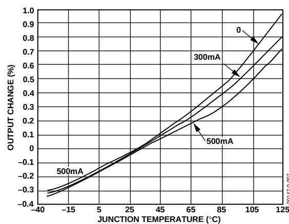
Figure 9. Output Voltage Variation vs. Junction Temperature
