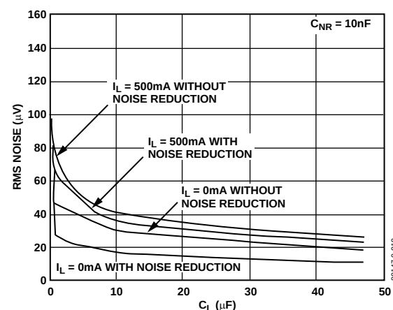
Figure 21. RMS Noise versus C_L (10 Hz to 100 kHz)
