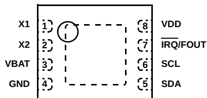
ISL1208 (8 LD TDFN) TOP VIEW
