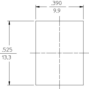
RECOMMENDED MOUNTING CUTOUT FOR \frac{.063}{1.6} THICK PANEL
