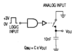
Figure 2. Charge Injection
