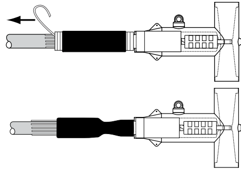
Typical Installation of ELB-600-CES
