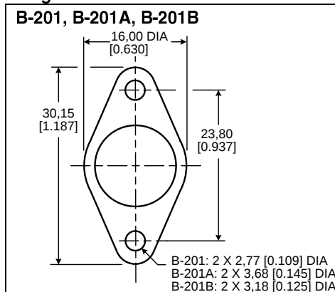
Figure 19. 3001/3004 Brackets
