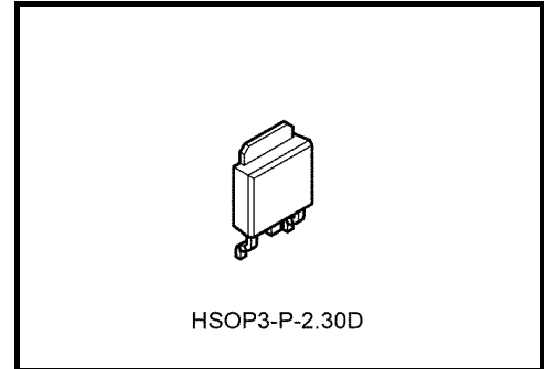
Weight HSOP3-P-2.30D: 0.36 g (typ.)
