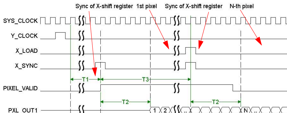
Figure 24. Pixel Output
