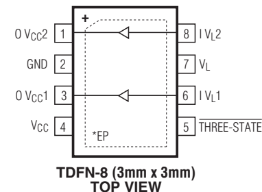
TDFN-8 (3mm x 3mm) TOP VIEW
