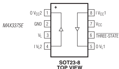
SOT23-8 TOP VIEW
