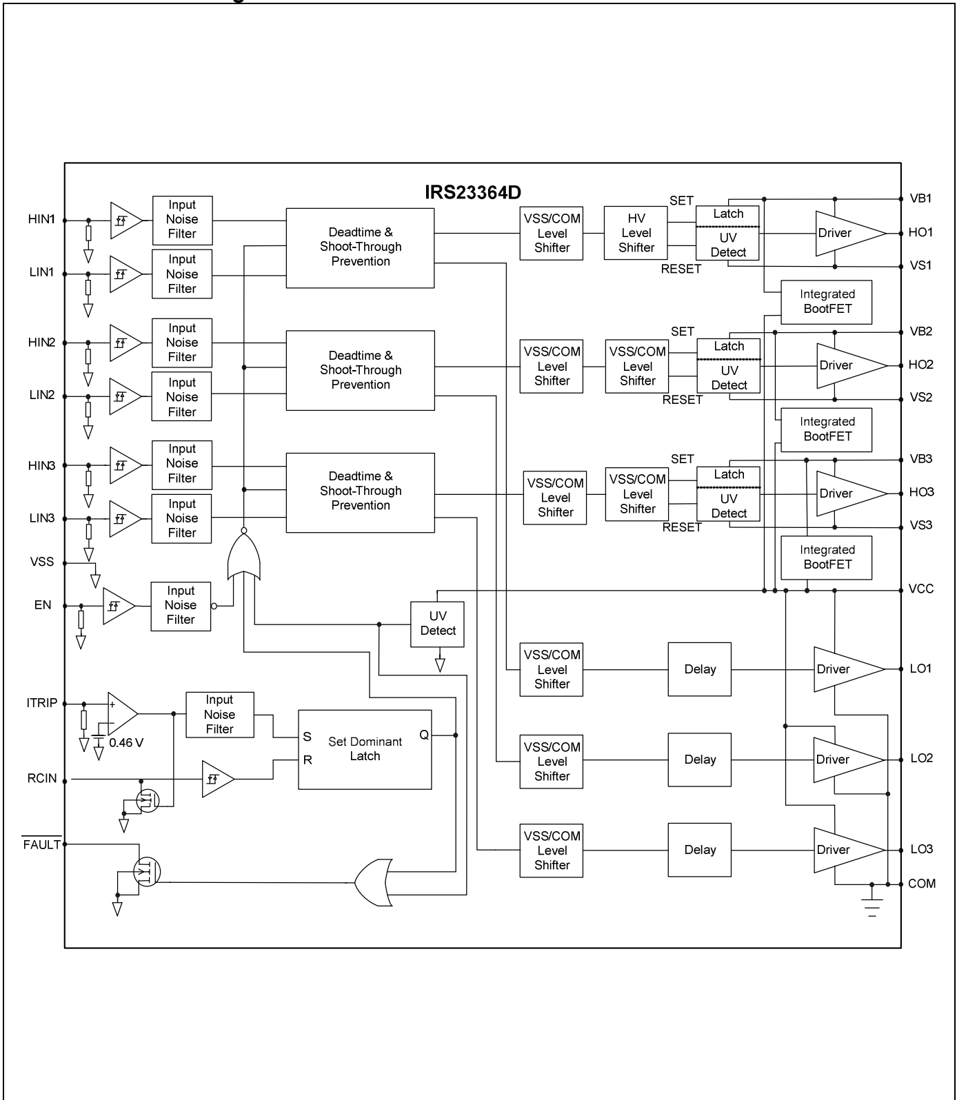
Functional Block Diagram: IRS23364D
