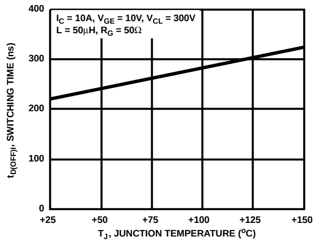
FIGURE 10. TYPICAL TURN-OFF DELAY TIME
