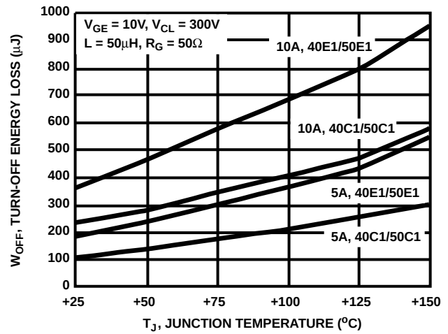
FIGURE 14. TYPICAL CLAMPED INDUCTIVE TURN-OFF SWITCHING LOSS/CYCLE
