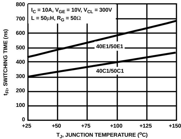
FIGURE 13. TYPICAL FALL TIME ( I_C = 10A )
