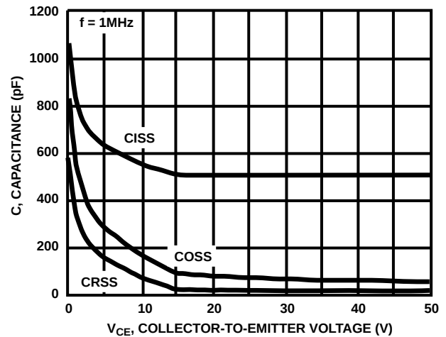
FIGURE 8. CAPACITANCE vs COLLECTOR-TO-EMITTER VOLTAGE
