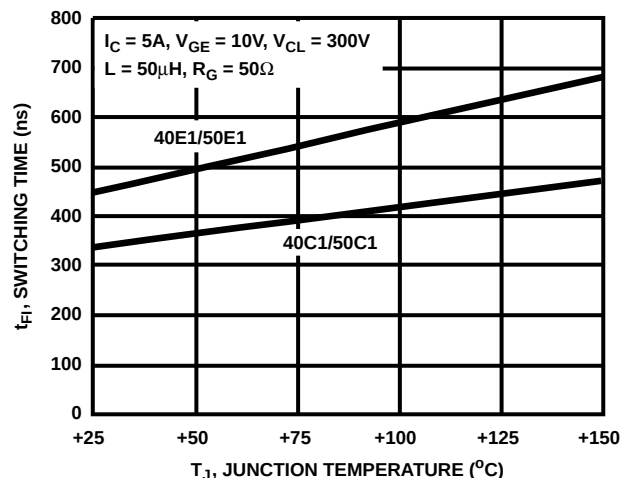
FIGURE 12. TYPICAL FALL TIME ( I_C = 5A )
