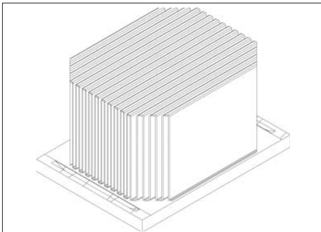
Figure 34. Mechanical Representation of the Boxed Processor Passive Heatsink
