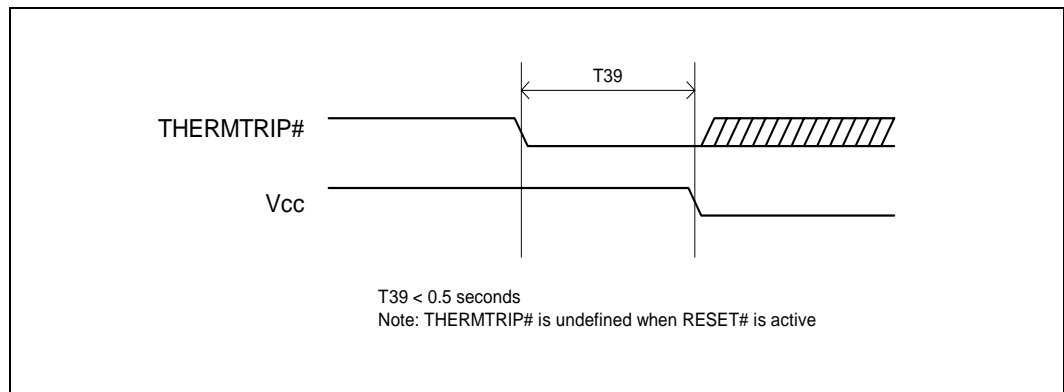
Figure 13. THERMTRIP# Power Down Waveform
