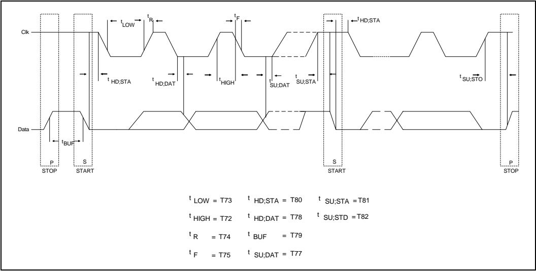
Figure 15. SMBus Valid Delay Timing Waveform
