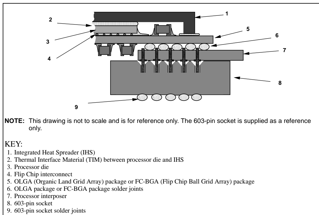
Figure 22. Processor Assembly Drawing (Including Socket)
