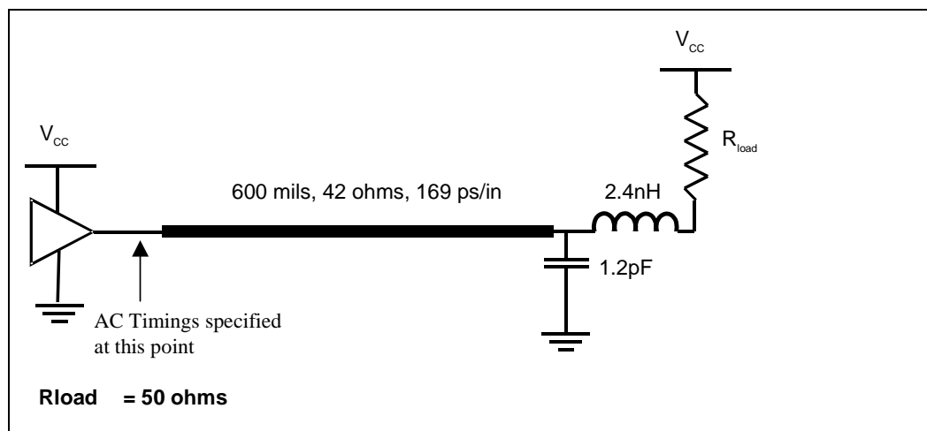
Figure 3. Electrical Test Circuit
