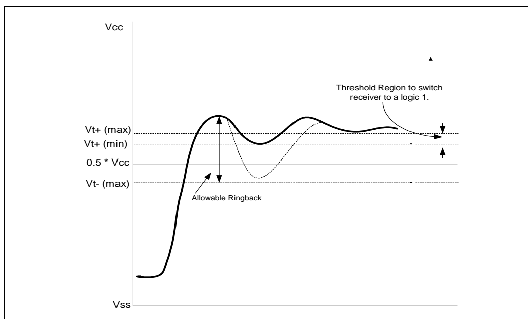
Figure 19. Low-to-High Receiver Ringback Tolerance for TAP Buffers
