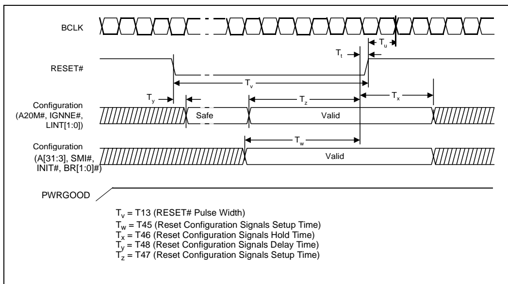
Figure 9. System Bus Reset and Configuration Timing Waveform
