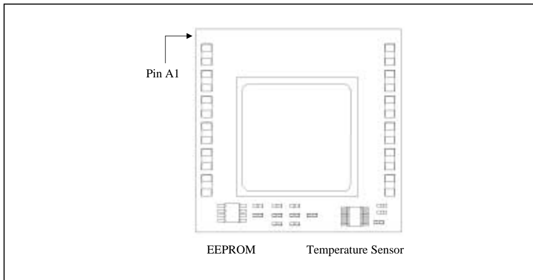
Figure 23. Top View Component Placement Detail
