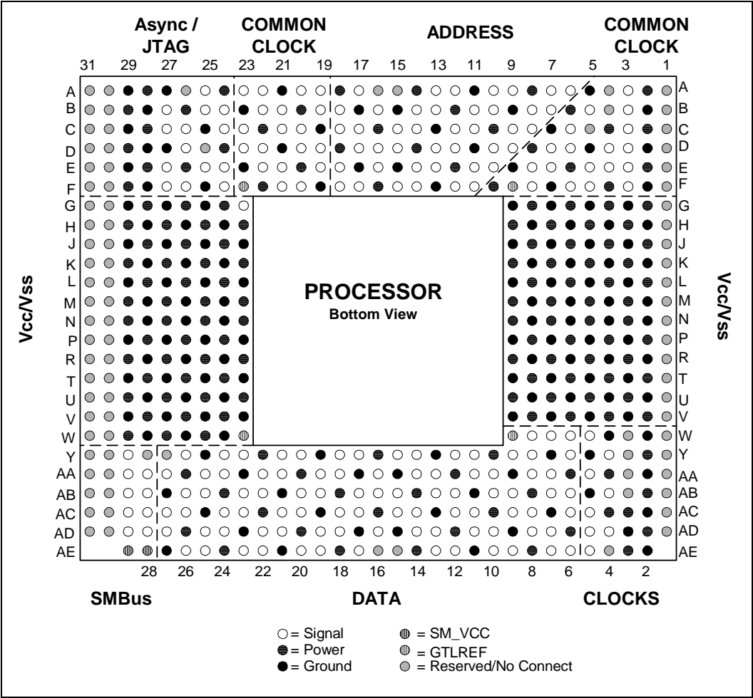
Figure 32. Processor Pin-out Diagram -- Bottom View
