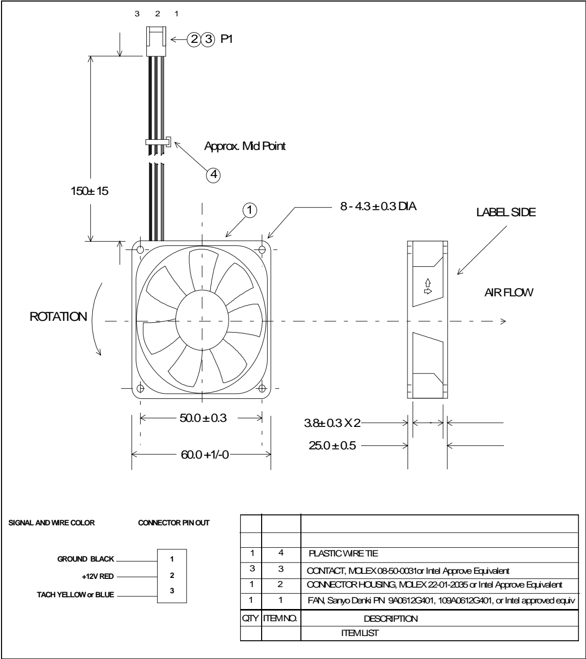
Figure 37. Boxed Processor Fan Power Cable Connector Description
