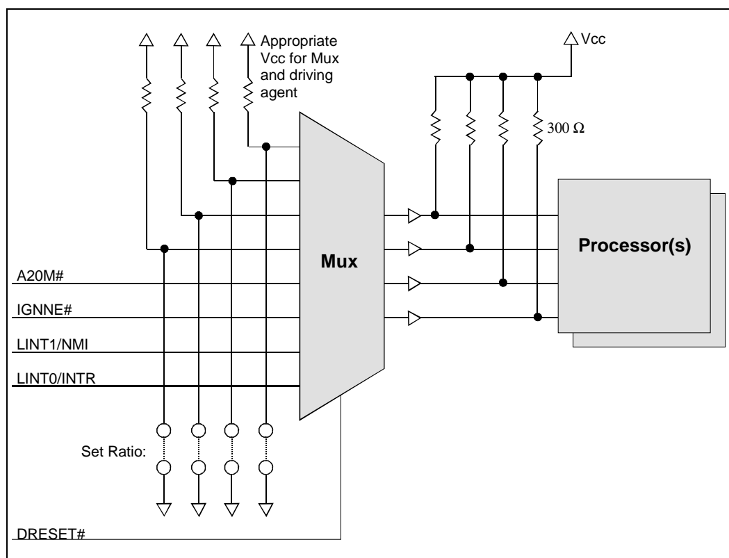
Figure 41. Example Schematic for Clock Ratio Pin Sharing
