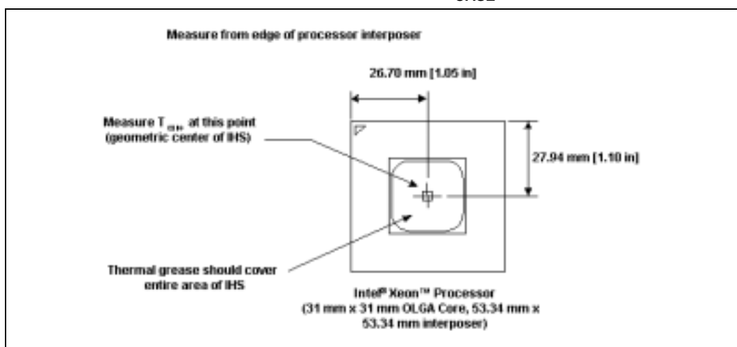
Figure 31. Thermocouple Placement for Case Temperature ( T_{CASE} ) Measurement
