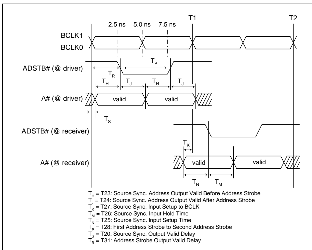
Figure 7. System Bus Source Synchronous 2X (Address) Timing Waveform
