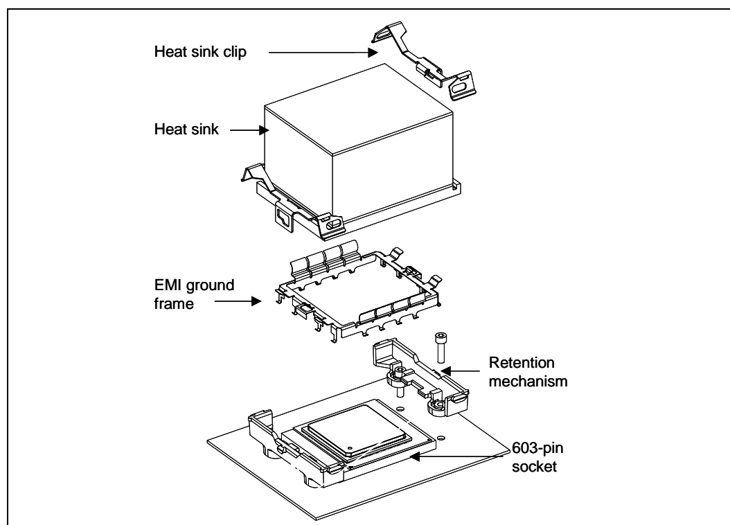
Figure 30. Processor with Thermal and Mechanical Components - Exploded View
