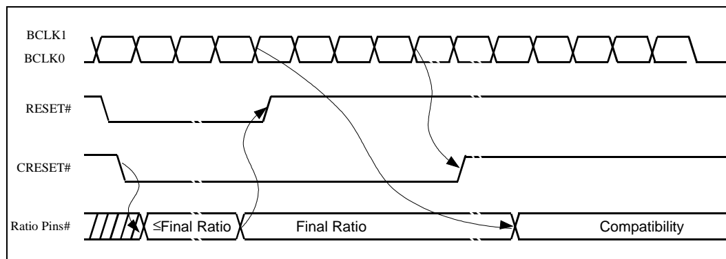
Figure 40. Timing Diagram of the Clock Ratio Signals
