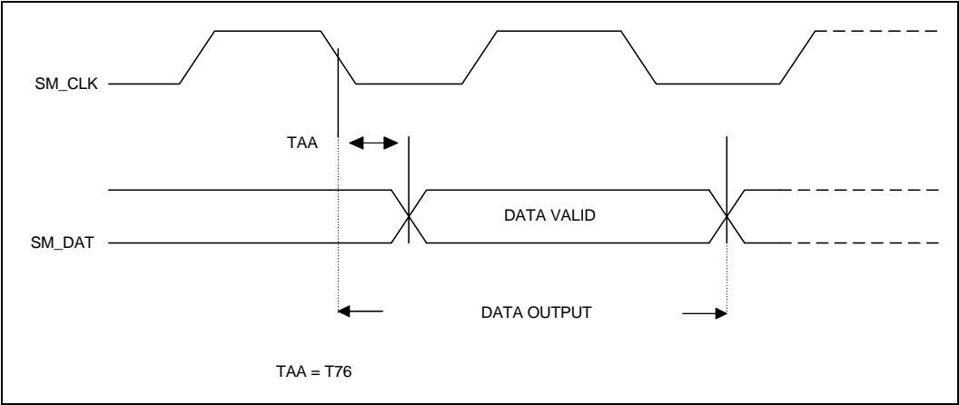
Figure 15. SMBus Valid Delay Timing Waveform
