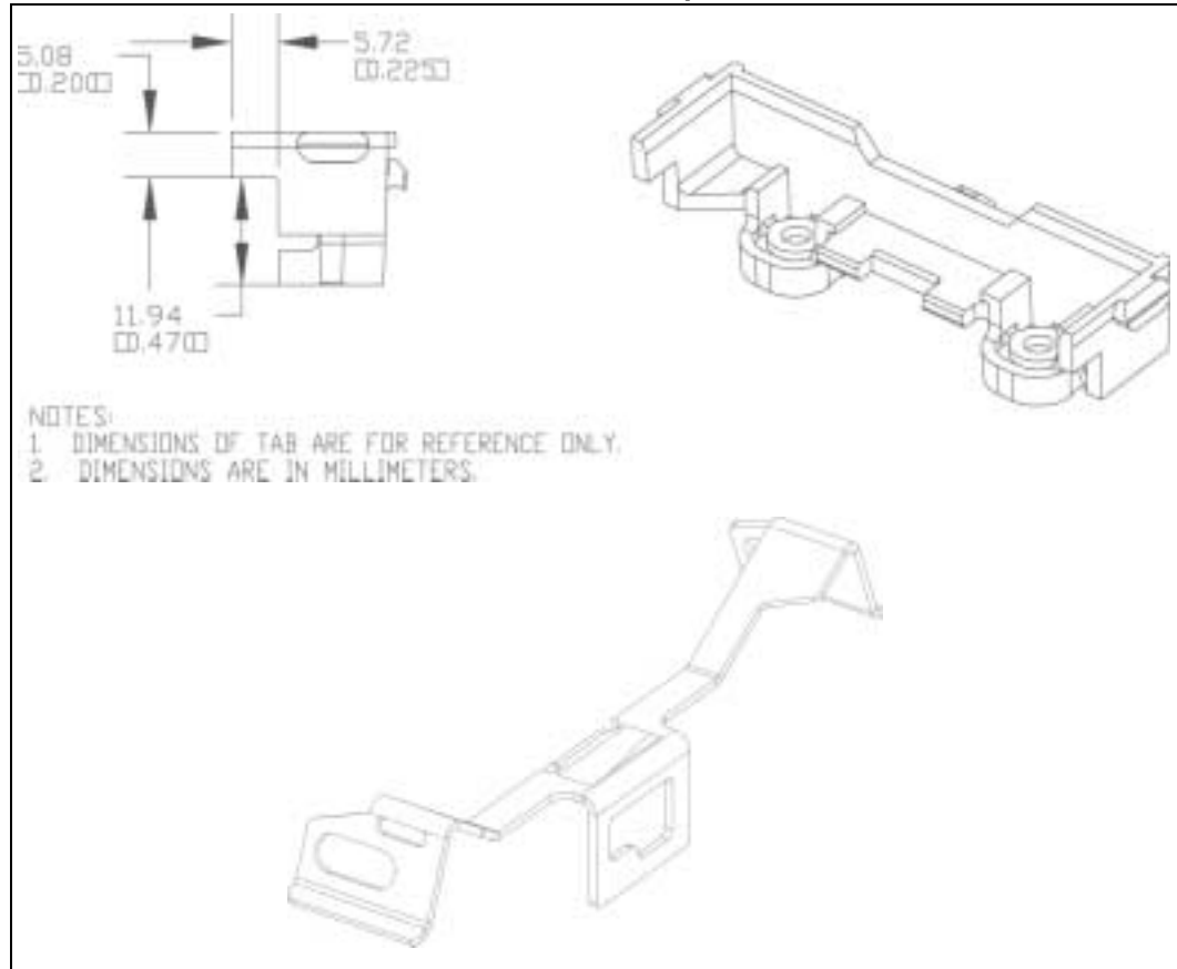
Figure 35. Boxed Processor Retention Mechanism and Clip
