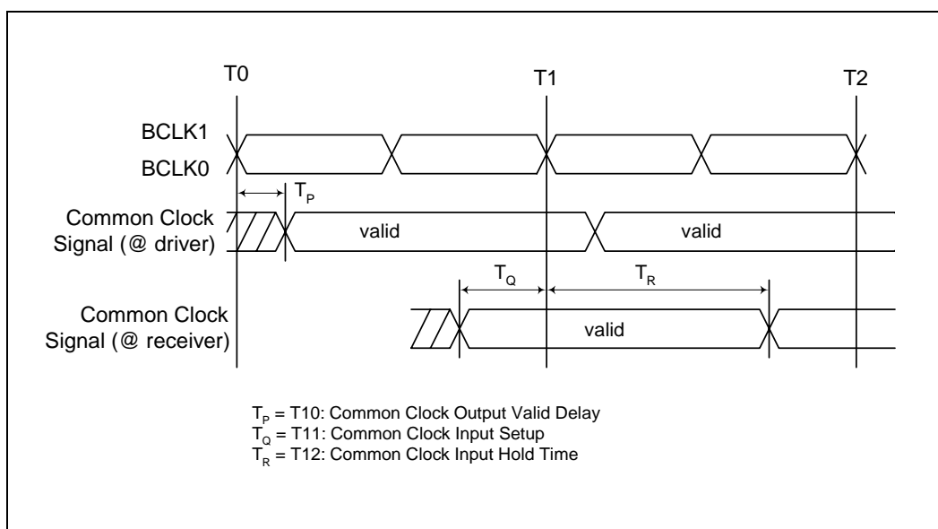
Figure 6. System Bus Common Clock Valid Delay Timing Waveform
