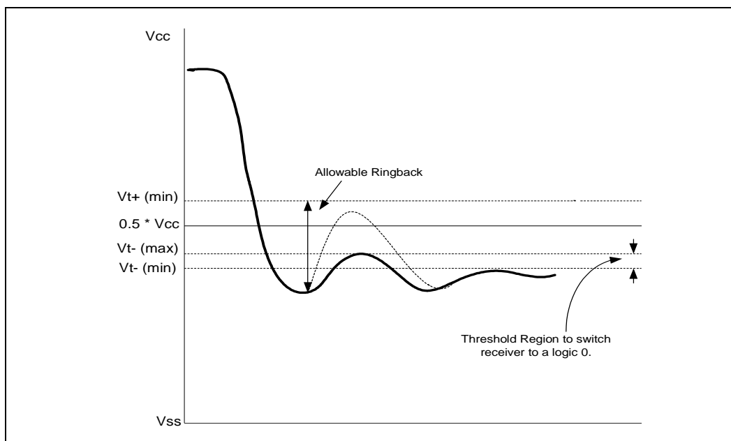
Figure 20. High-to-Low Receiver Ringback Tolerance for TAP Buffers
