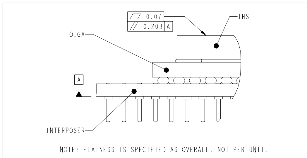
Figure 28. IHS Flatness and Tilt Drawing
