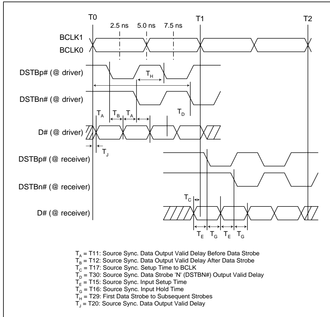
Figure 8. System Bus Source Synchronous 4X (Data) Timing Waveform
