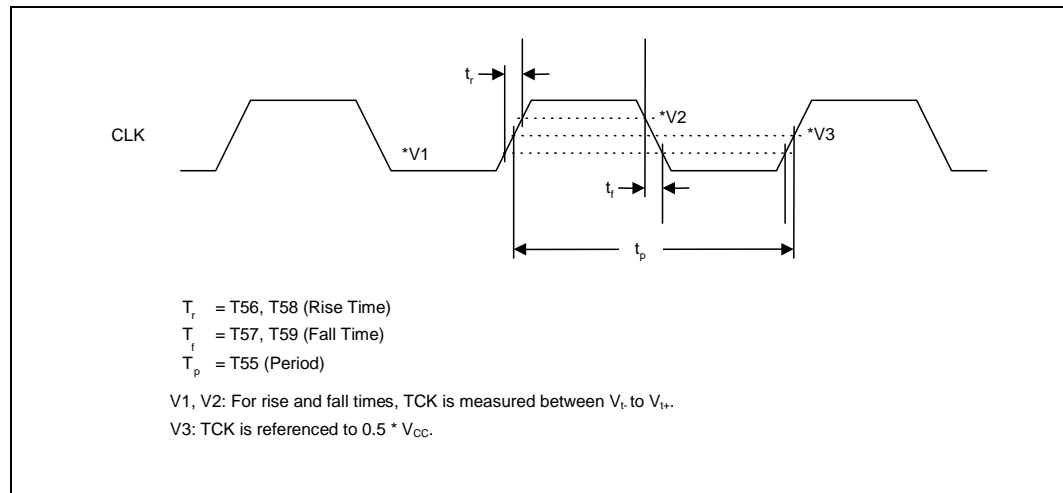
Figure 4. TCK Clock Waveform
