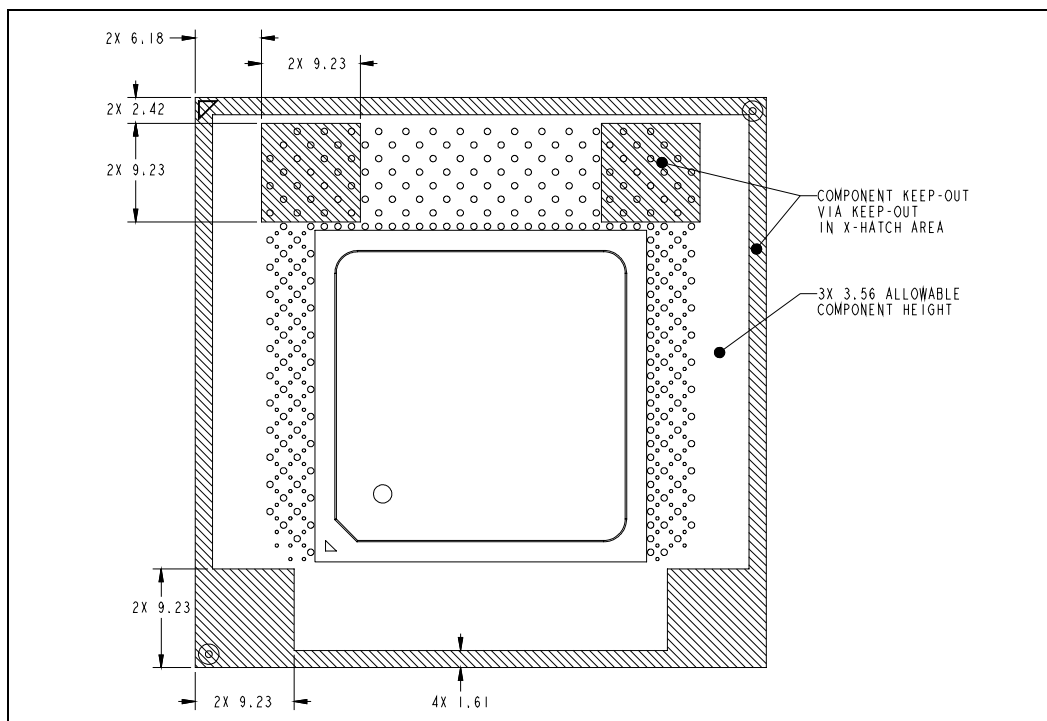
Figure 25. Top View - Component Height Keep-in
