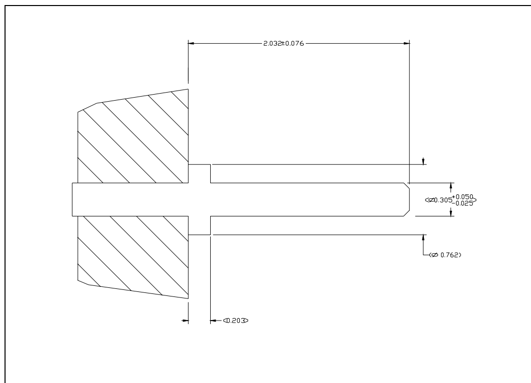
Figure 27. Processor Pin Detail
