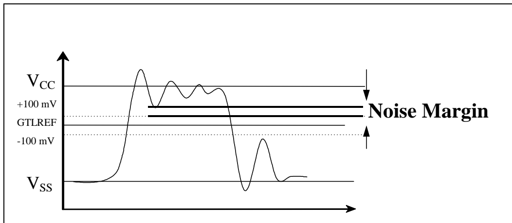
Figure 18. High-to-Low Receiver Ringback Tolerance for AGTL+ and Async GTL+ Signals
