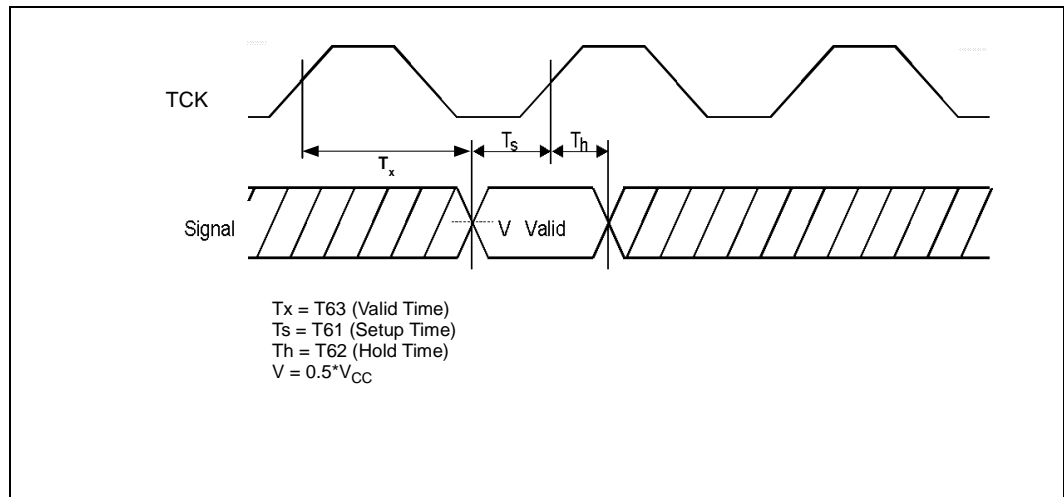
Figure 12. Test Reset (TRST#), Async GTL+ Input, and PROCHOT# Timing Waveform
