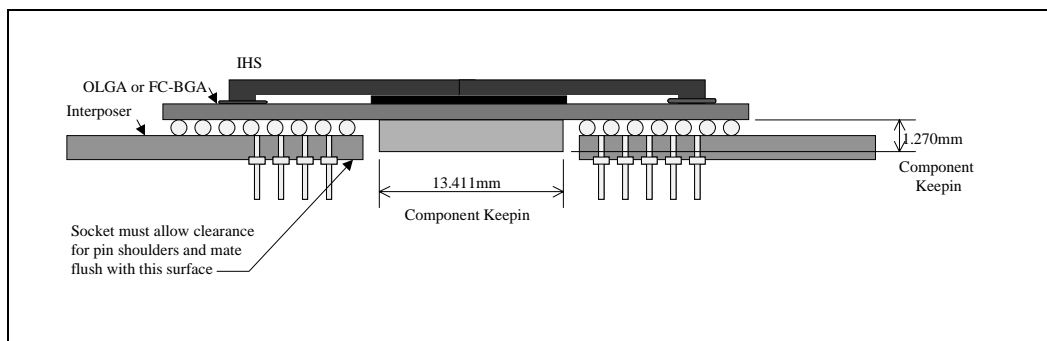
Figure 26. Processor Cross Section View - Pin Side Component Keep-in
