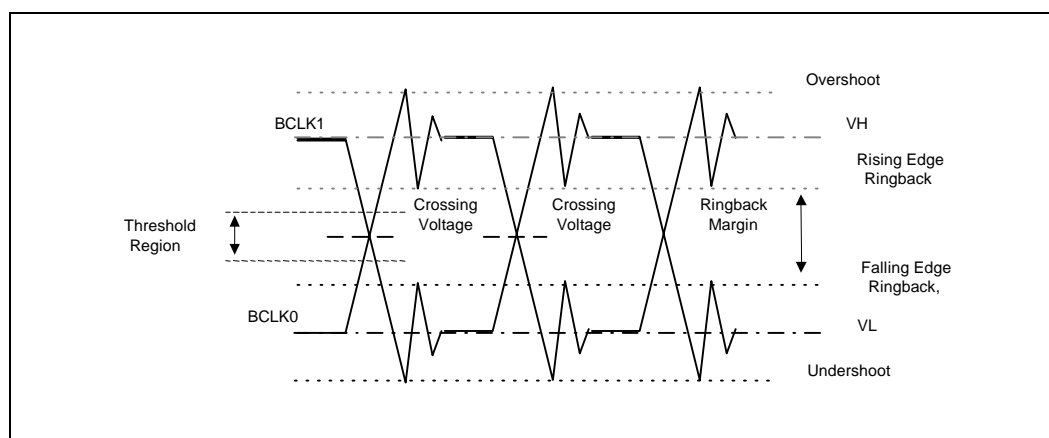
Figure 16. BCLK[1:0] Signal Integrity Waveform
