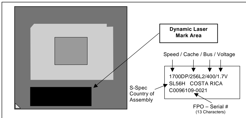
Figure 30. Processor Bottom-Side Markings
