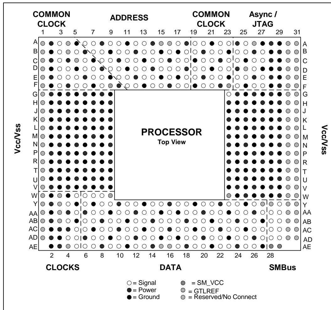
Figure 31. Processor Pin-out Diagram -- Top View
