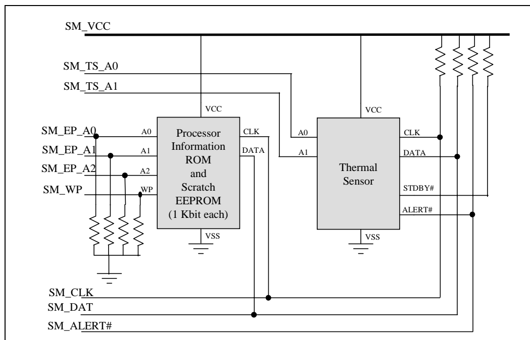
Figure 33. Logical Schematic of SMBus Circuitry
