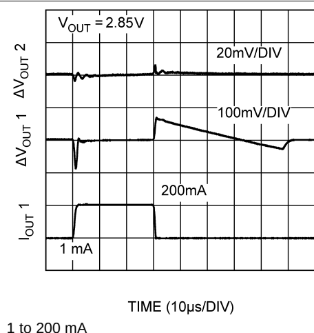
Figure 13. OUT1 Load Transient
