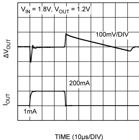
Figure 15. Load Transient
