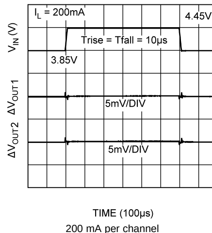
Figure 16. Line Transient
