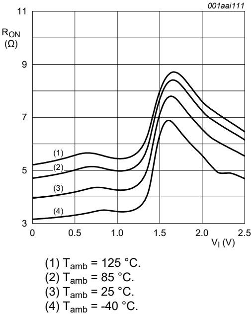
Fig. 8. ON resistance as a function of input voltage; V_{CC} = 2.5\text{ V}; I_{SW} = 64\text{ mA}
