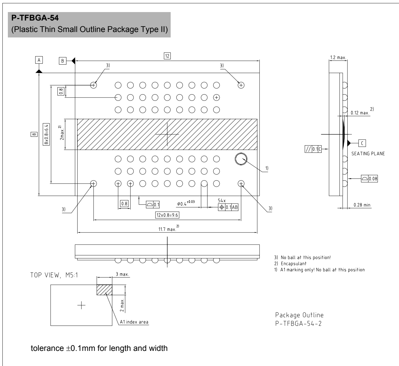
Figure 3 Package Outline
