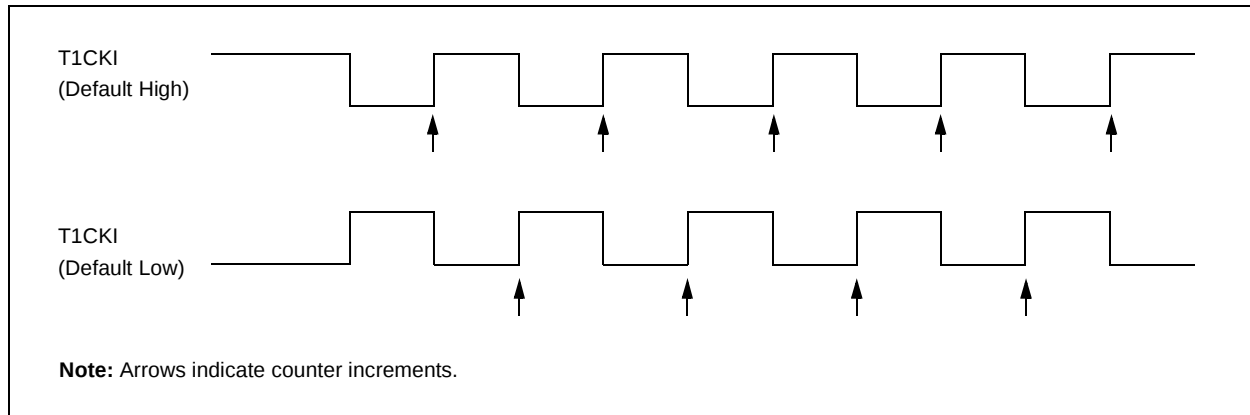
FIGURE 6-1: TIMER1 INCREMENTING EDGE
