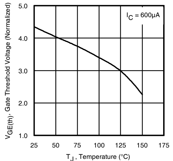
Fig. 23 - Typical Gate Threshold Voltage (Normalized) vs. Junction Temperature I_C = 600\mu\text{A}
