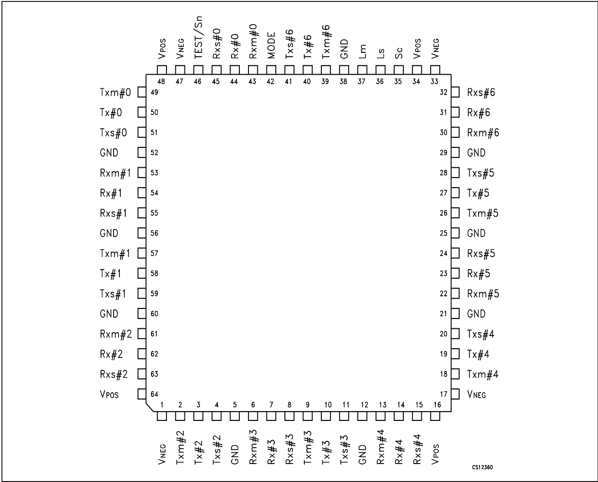
Figure 2. Pin configuration
