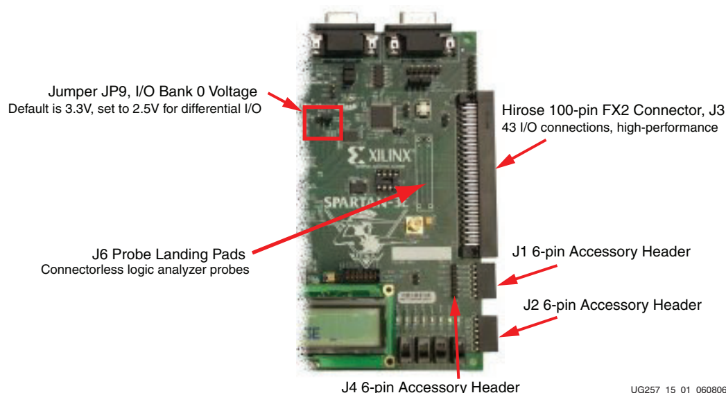
Figure 15-1: Expansion Headers
