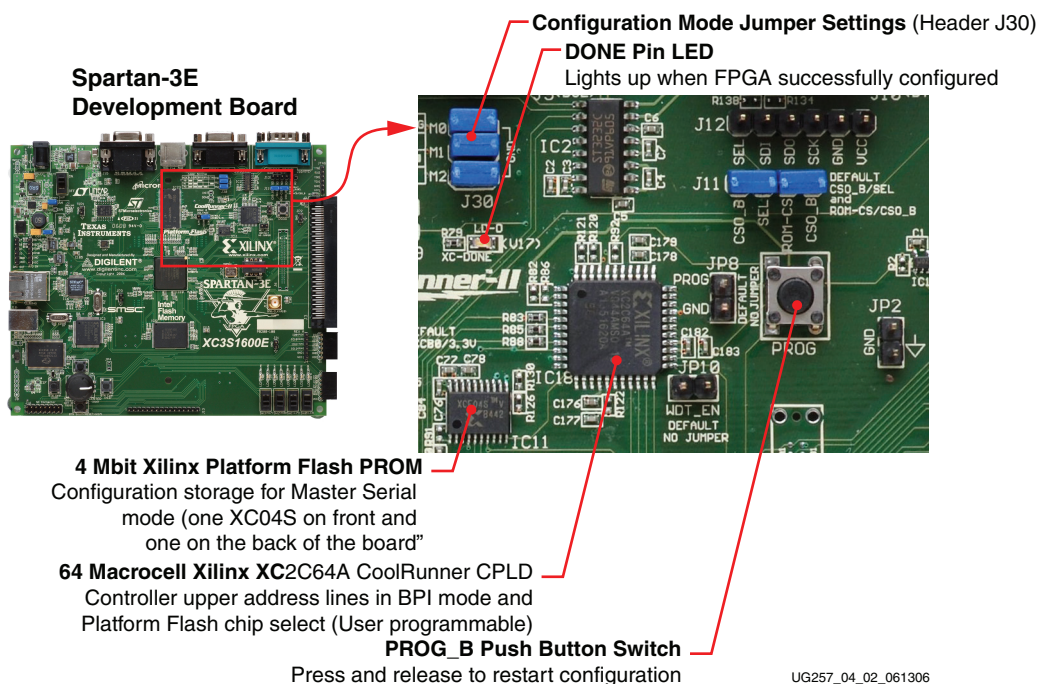
Figure 4-2: Detailed Configuration Options
