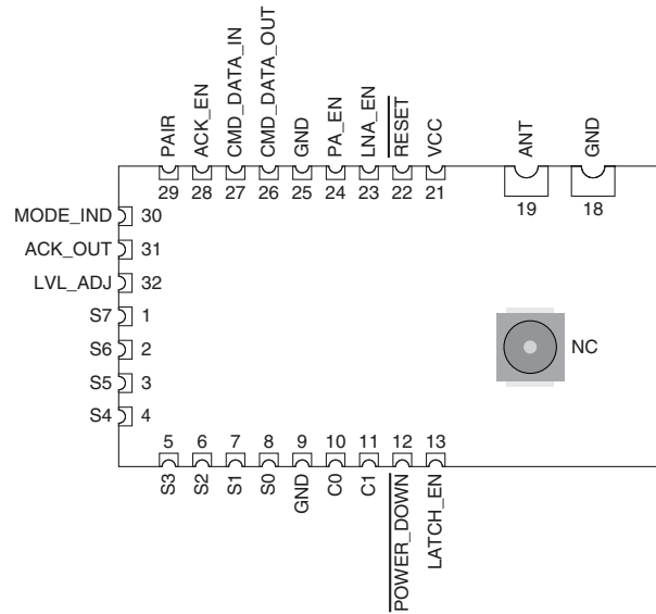
Figure 28: HumRC™ Series Transceiver Pre-certified Version Pin Assignments - Castellated Connection (Top View)
