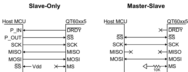
Figure 4-1 SPI Connections
