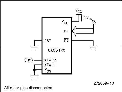
Figure 8. I_{CC} Test Condition, Power Down Mode V_{CC} = 2.0\text{V to } 6.0\text{V}
