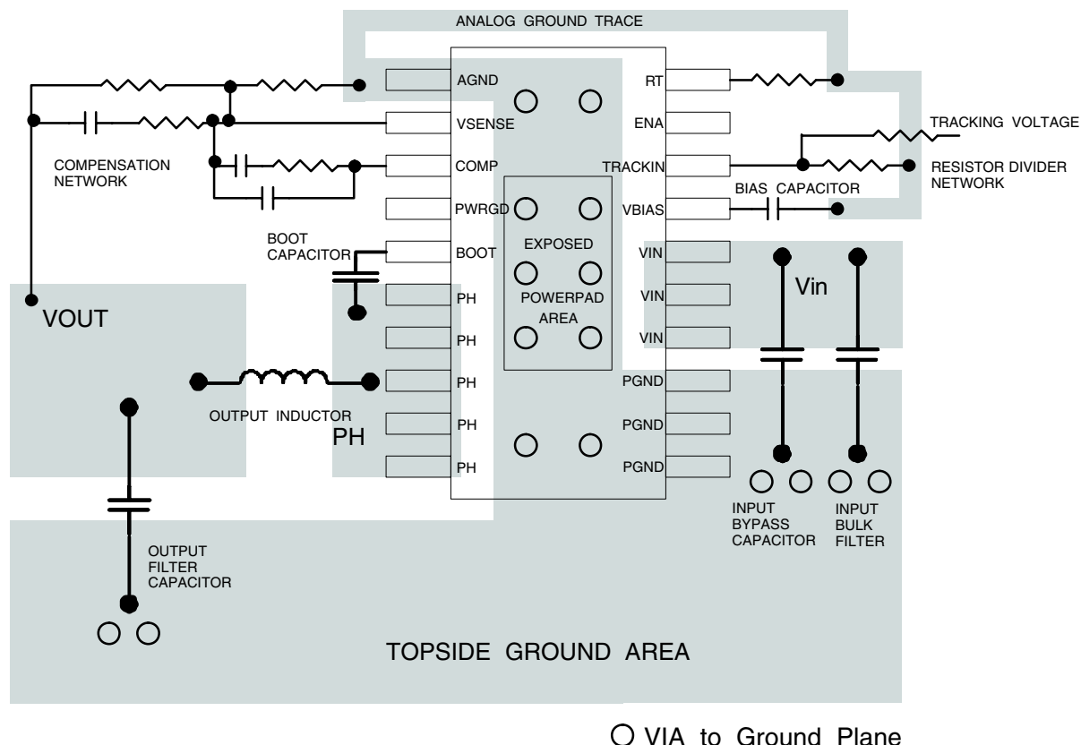
Figure 10. TPS54380 PCB Layout
