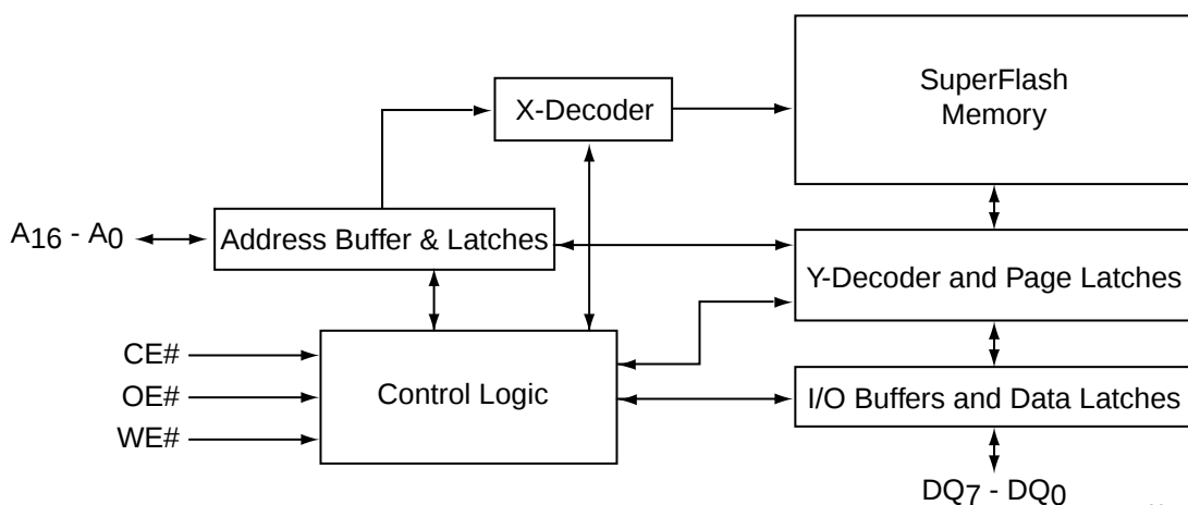
FUNCTIONAL BLOCK DIAGRAM OF SST29EE010/29LE010/29VE010
