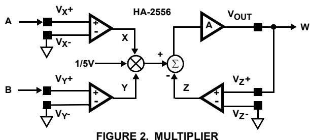
FIGURE 2. MULTIPLIER
