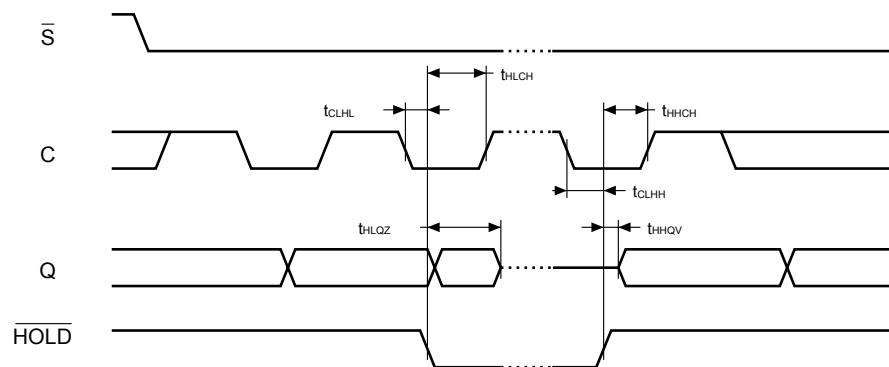
Figure 20. Hold timing
