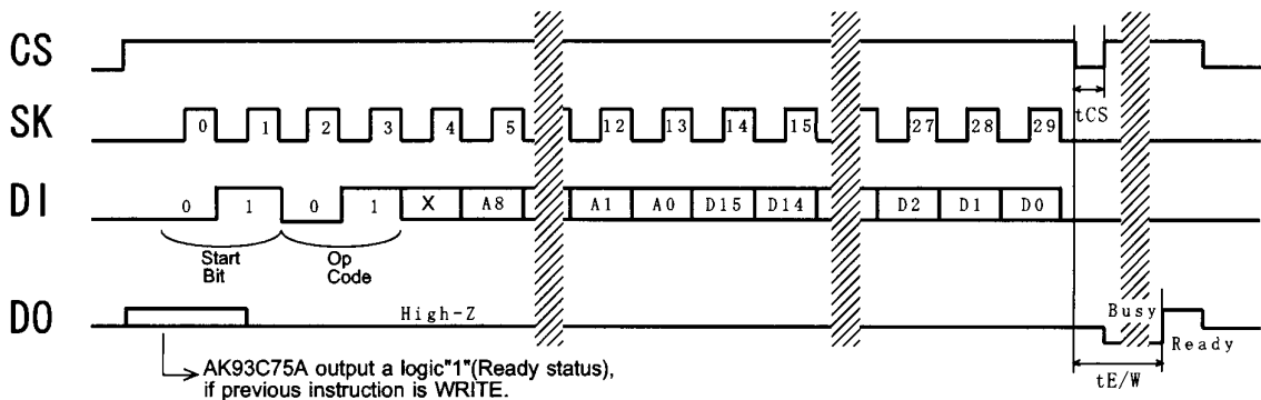
WRITE (AK93C75A)
