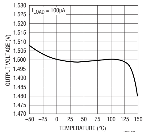
Output Voltage LT3008-1.5
