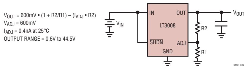
Figure 2. Adjustable Operation
