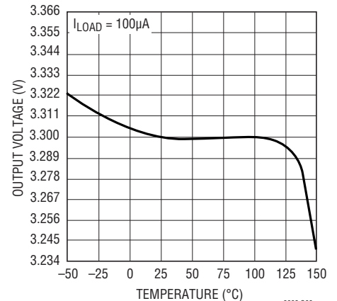
Output Voltage LT3008-3.3
