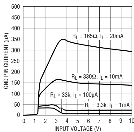
GND Pin Current LT3008-3.3
