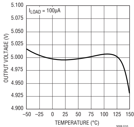
Output Voltage LT3008-5
