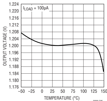
Output Voltage LT3008-1.2
