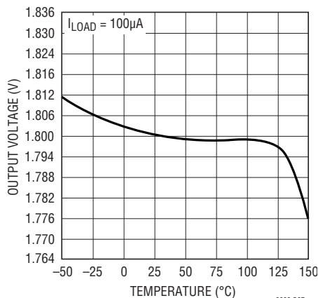
Output Voltage LT3008-1.8
