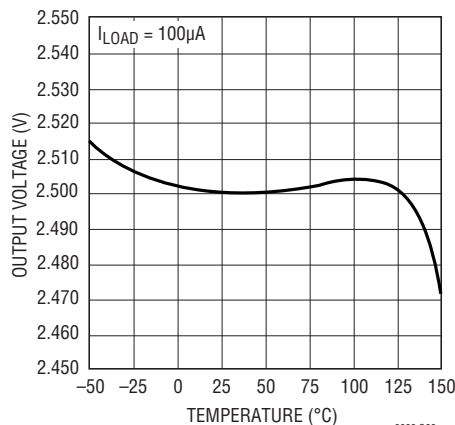
Output Voltage LT3008-2.5
