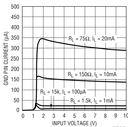
GND Pin Current LT3008-1.5
