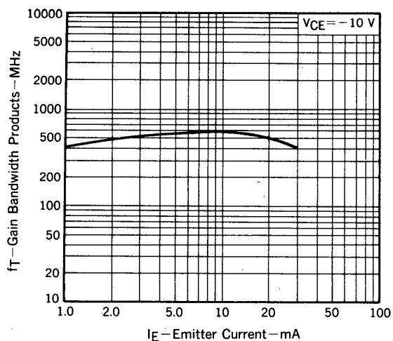
GAIN BANDWIDTH PRODUCTS vs. EMITTER CURRENT
