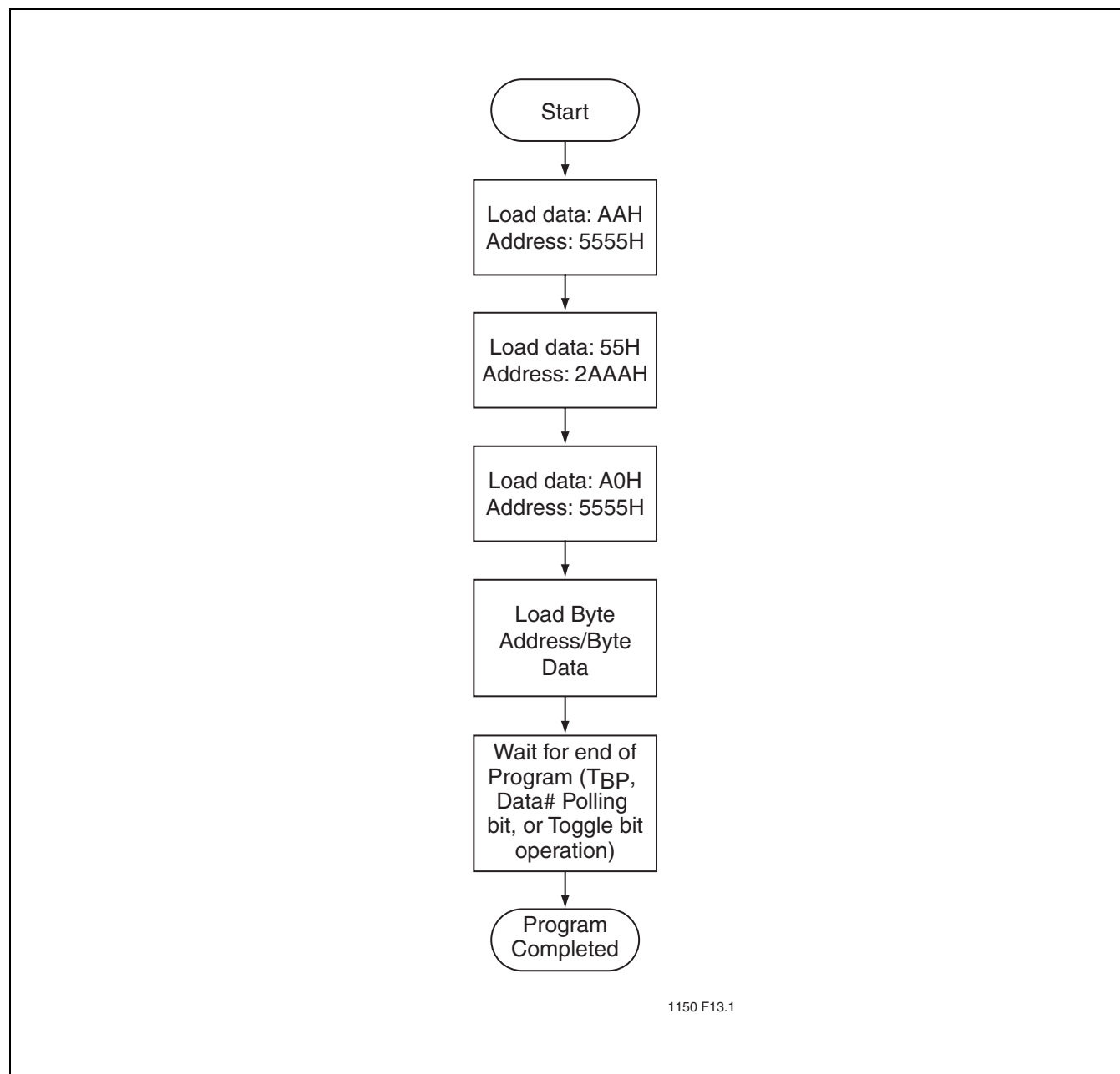
FIGURE 17: Byte-Program Algorithm
