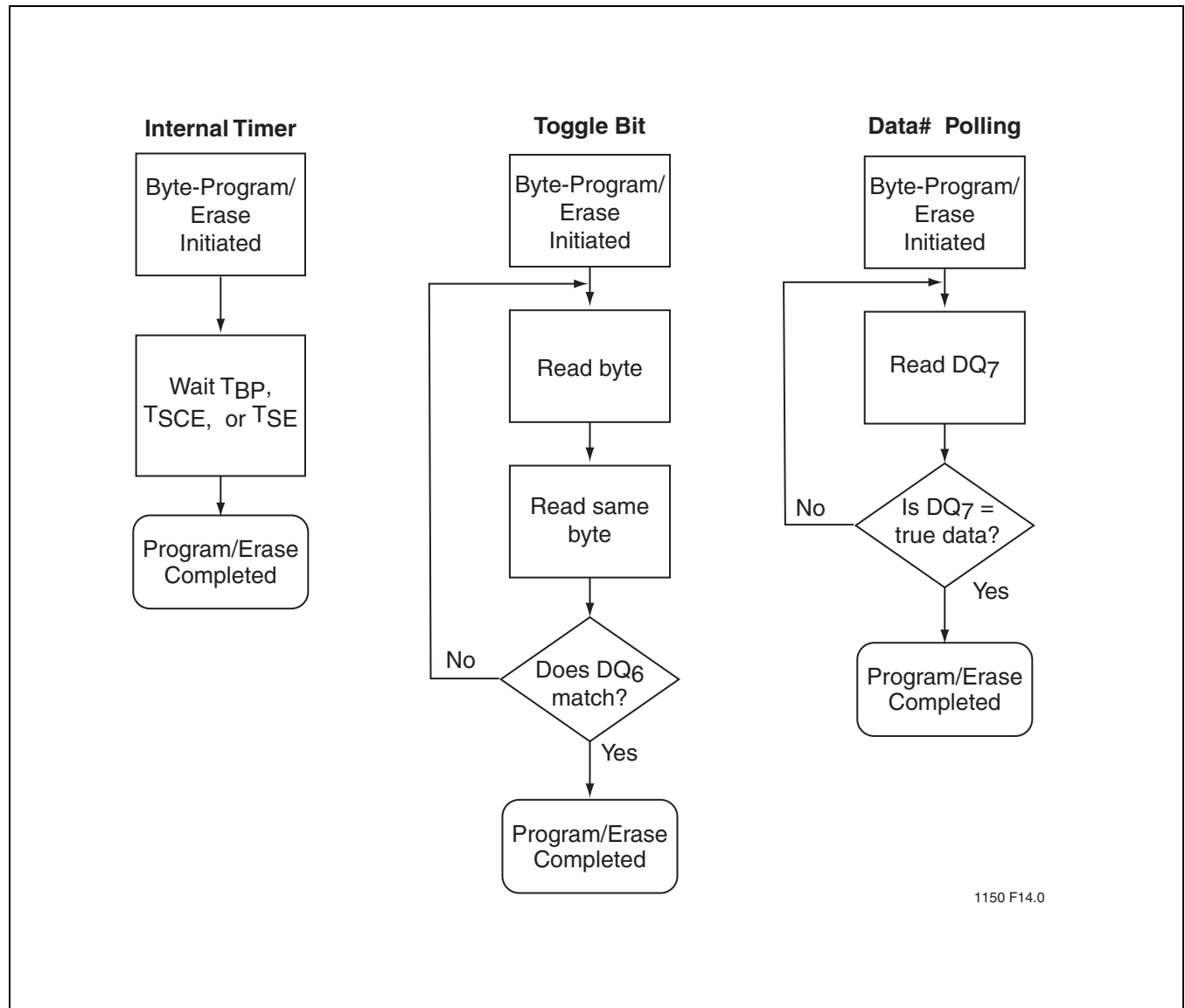
FIGURE 18: Wait Options
