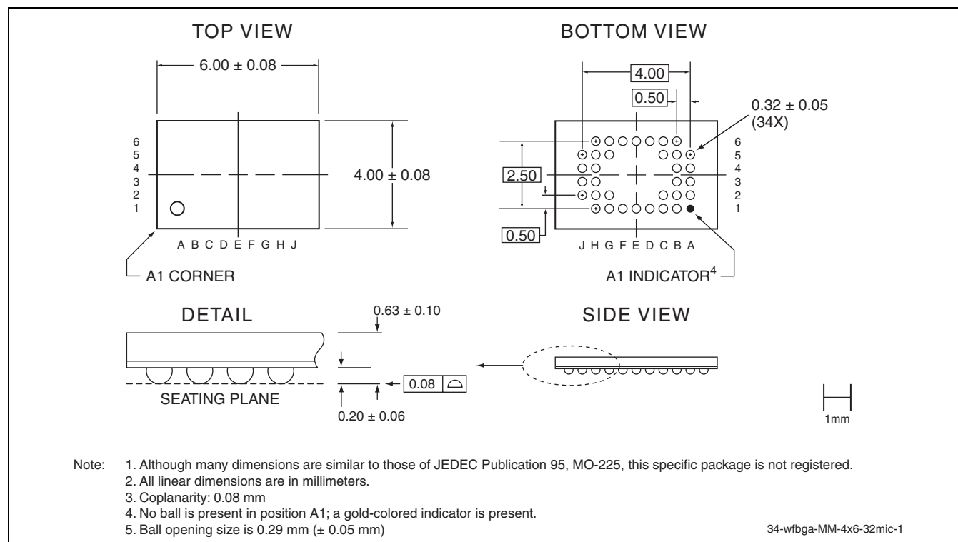
FIGURE 24: 34-ball Very-very-thin-profile, Fine-pitch Ball Grid Array (WFBGA) 4mm x 6mm x .63mm SST Package Code: MM
