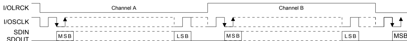
Figure 7. Serial Audio Interface Format - I²S
