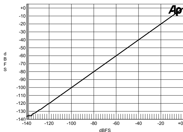
Figure 53. Linearity Error, 0 to -140 dBFS Input, 200 Hz Tone, 96 kHz:48 kHz
