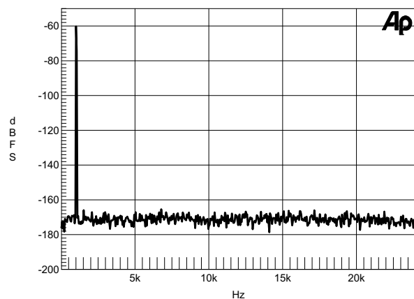
Figure 25. Wideband FFT Plot (16k Points) -60 dBFS 1 kHz Tone, 44.1 kHz:48 kHz
