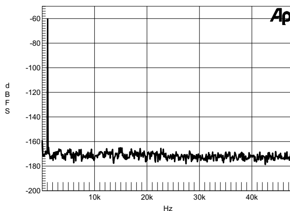
Figure 22. Wideband FFT Plot (16k Points) -60 dBFS 1 kHz Tone, 48 kHz:96 kHz
