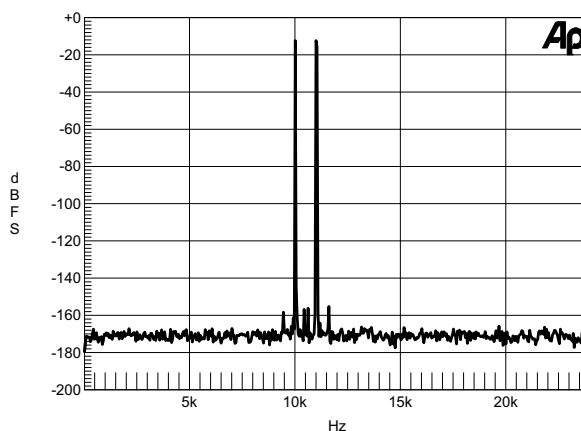
Figure 28. IMD, 10 kHz and 11 kHz -7 dBFS, 96 kHz:48 kHz
