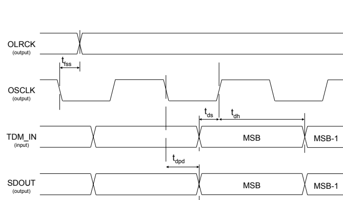
Figure 4. TDM Master Mode Timing
