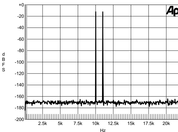
Figure 30. IMD, 10 kHz and 11 kHz -7 dBFS, 48 kHz:44.1 kHz
