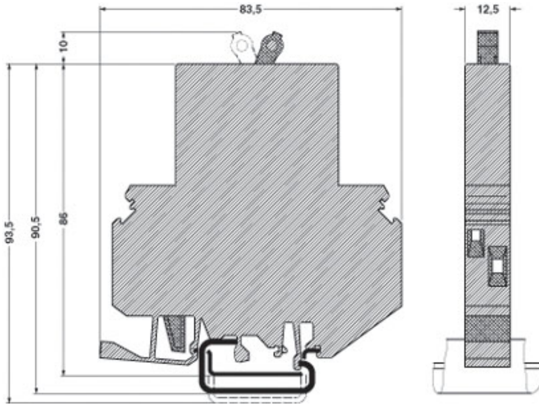
Dimensioned drawing
