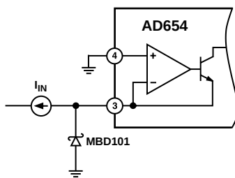
Figure 5. Input Protection
