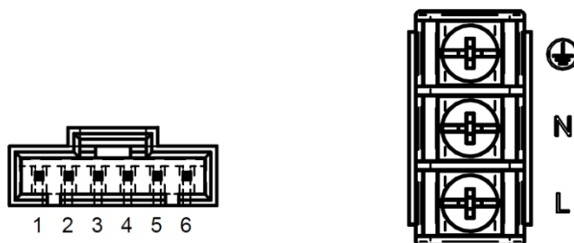
Figure 4. LPM409 Front Panel Connectors Pinout View
