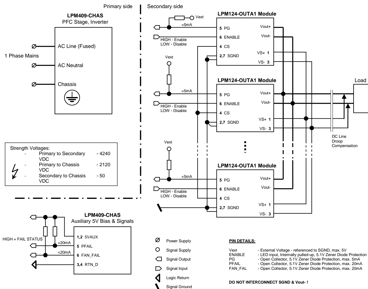
Figure 16. LPM409 – Connection Diagram
