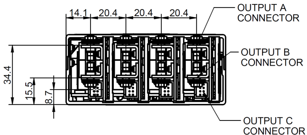
Figure 7. Rear View
