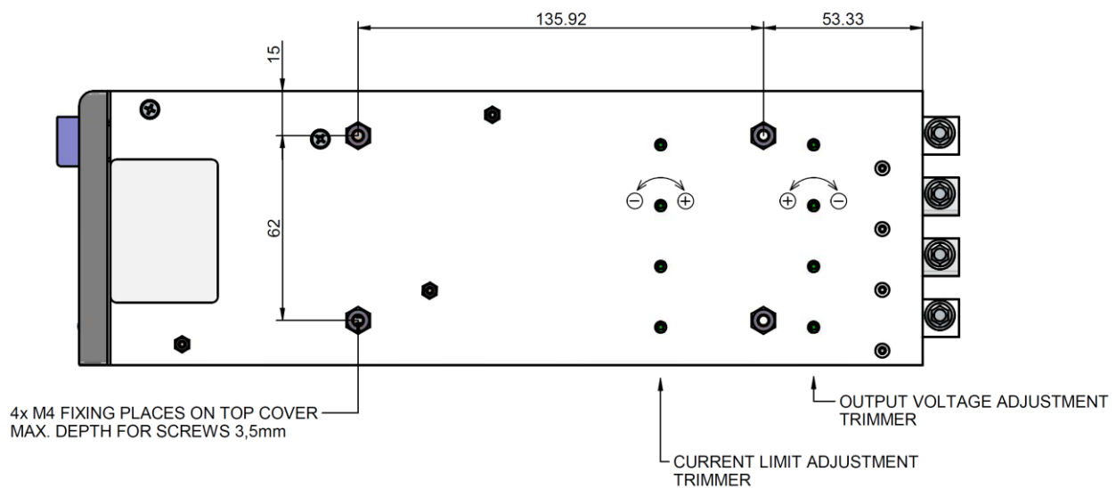
Figure 10. Bottom View
