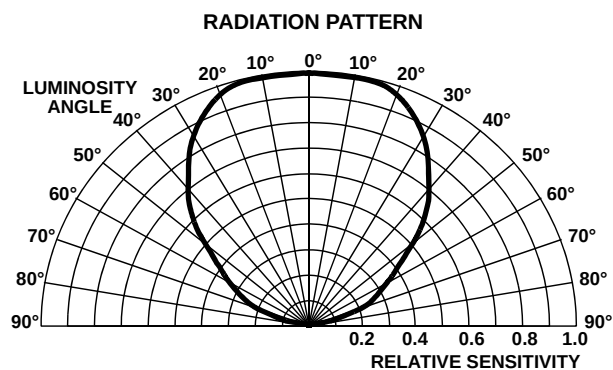
FIGURE 10. RADIATION PATTERN
