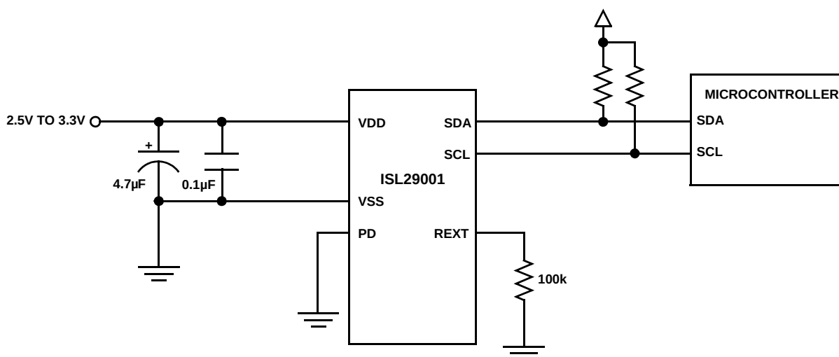
FIGURE 13. TYPICAL CIRCUIT
