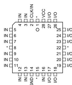
LCC/PLCC
