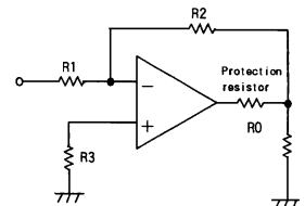
Fig.2 The example of protection resistor
