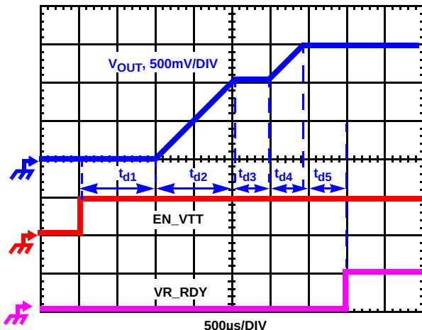
FIGURE 8. SOFT-START WAVEFORMS
