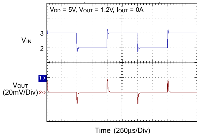
V_{IN} Line Transient Response
