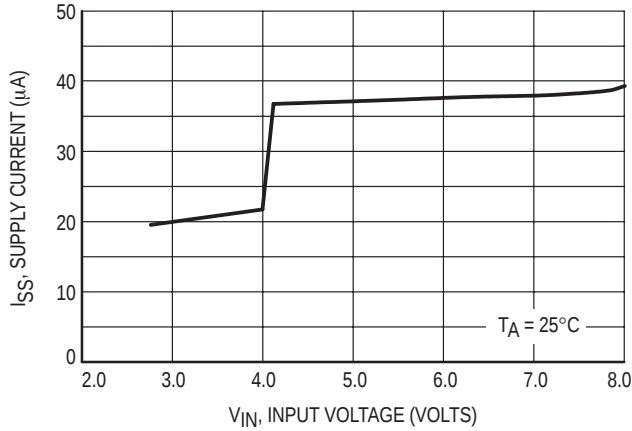
Figure 23. MC78PC40 (4.0 V) Supply Current versus Input Voltage
