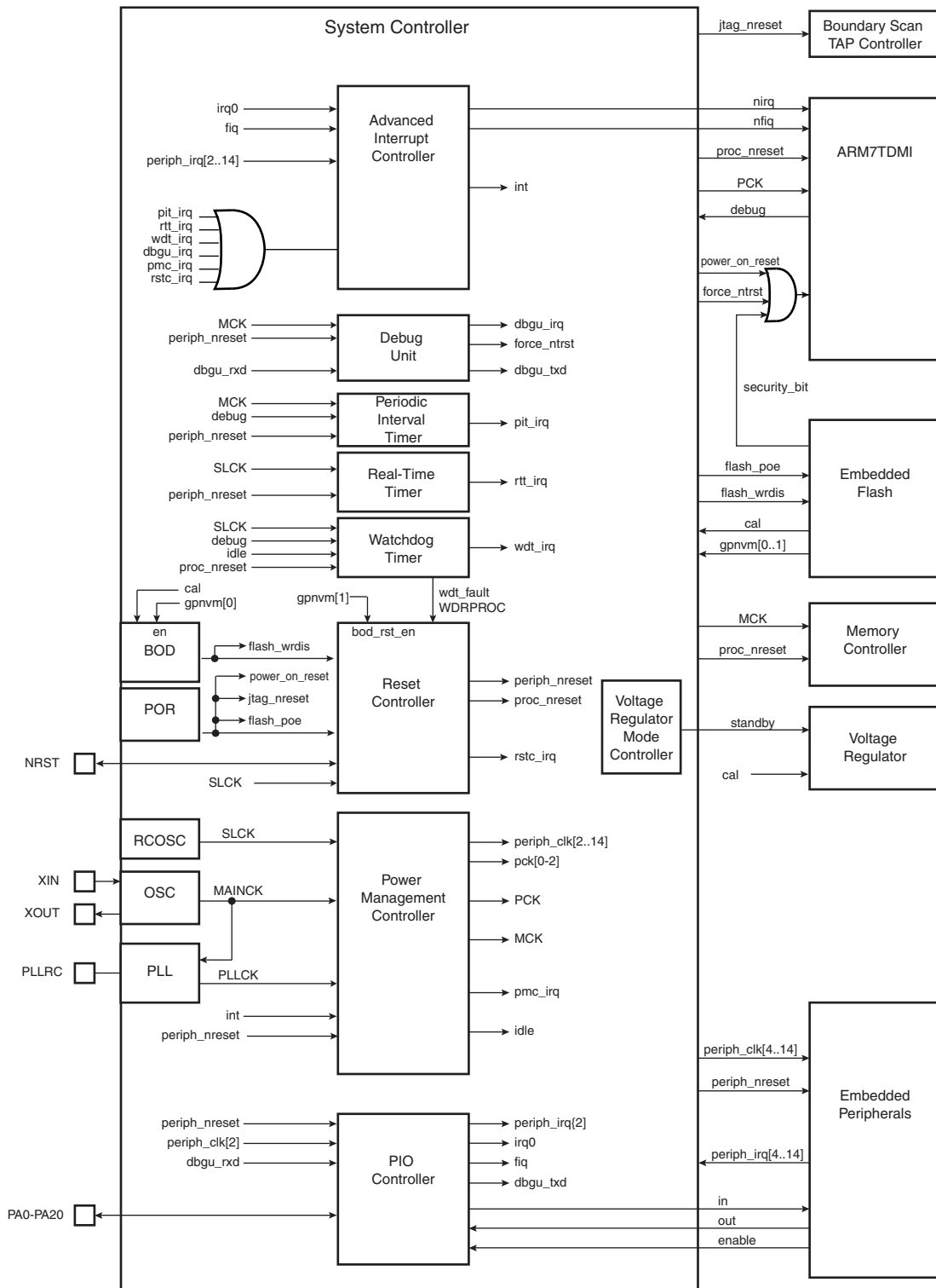
Figure 9-2. System Controller Block Diagram (AT91SAM7S32)
