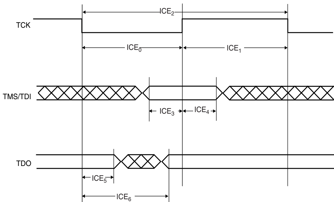
Figure 36-7. ICE Interface Signals
