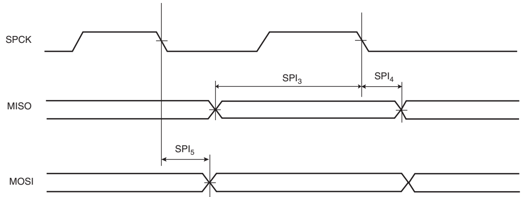
Figure 36-4. SPI Master mode with (CPOL=0 and NCPHA=1) or (CPOL=1 and NCPHA=0)
