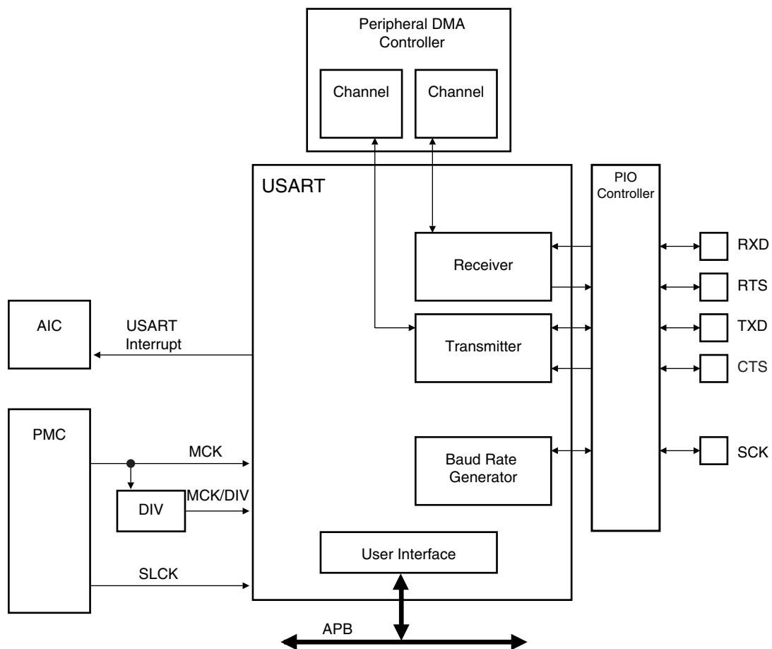
Figure 30-2. AT91SAM7S32 USART Block Diagram
