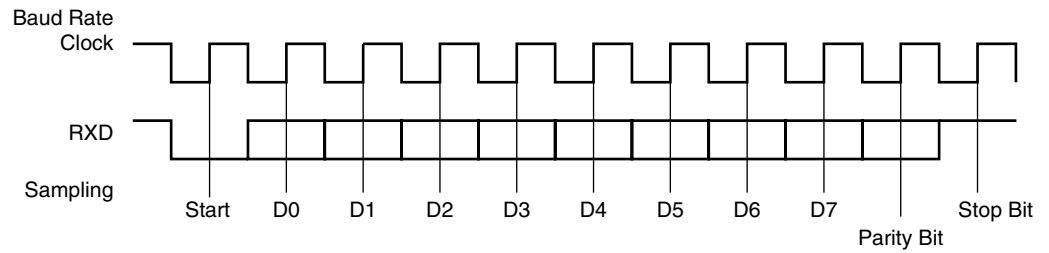
Figure 30-12. Synchronous Mode Character Reception
