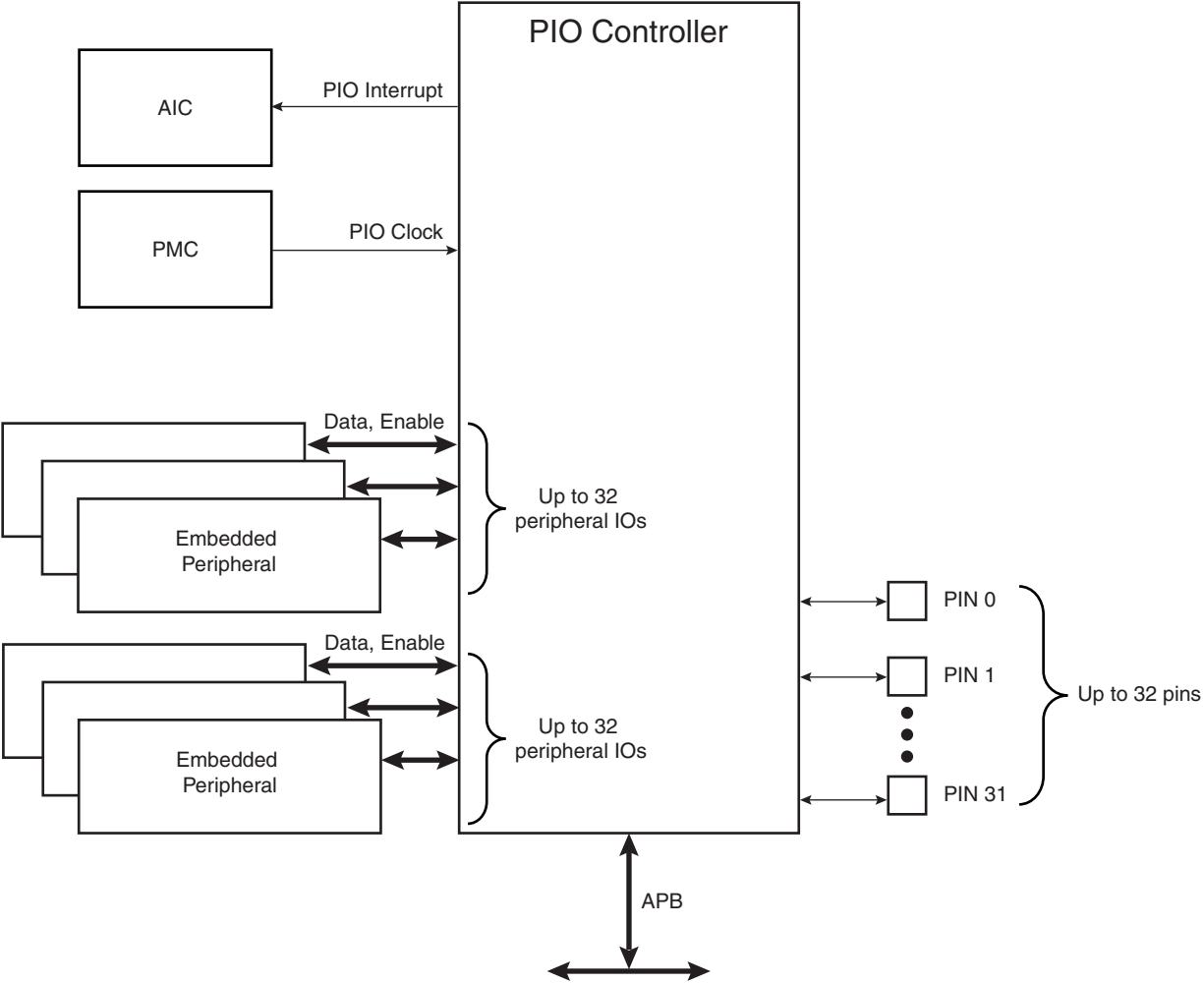
Figure 15-2. Application Block Diagram
