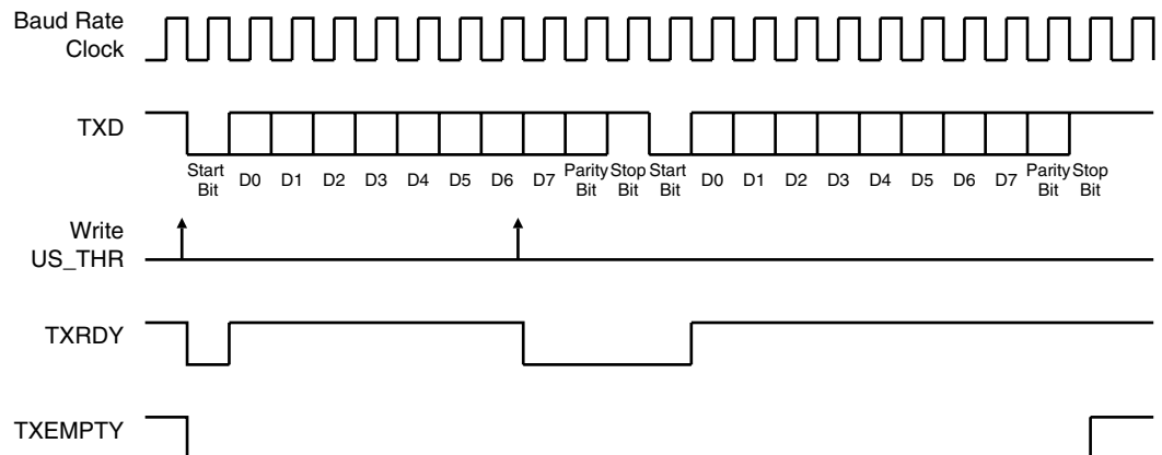
Figure 30-9. Transmitter Status
