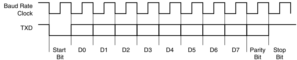
Figure 30-8. Character Transmit
