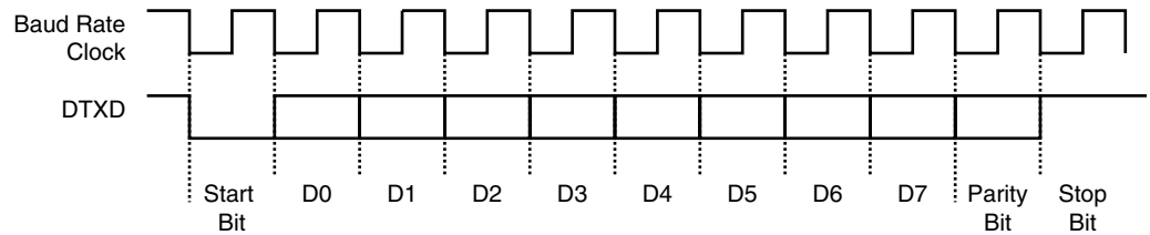
Figure 27-10. Character Transmission
