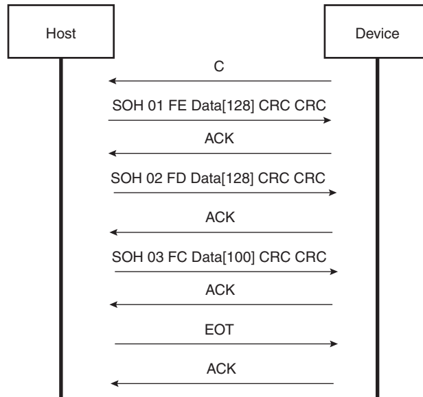
Figure 22-4. Xmodem Transfer Example
