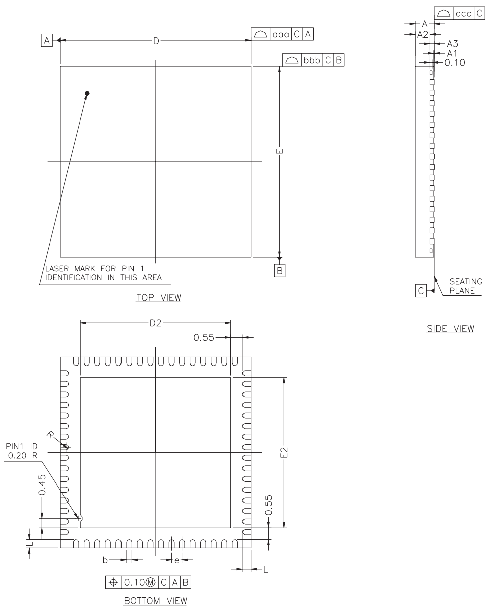
Figure 37-3. 64-pad QFN Package Drawing
