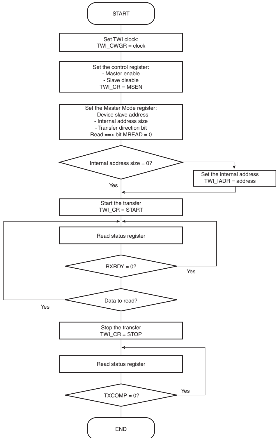
Figure 29-11. TWI Read in Master Mode
