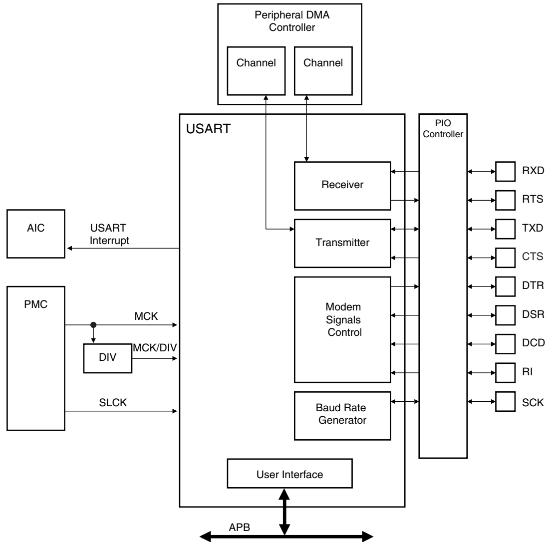
Figure 30-1. AT91SAM7S512/256/128/64/321 USART Block Diagram
