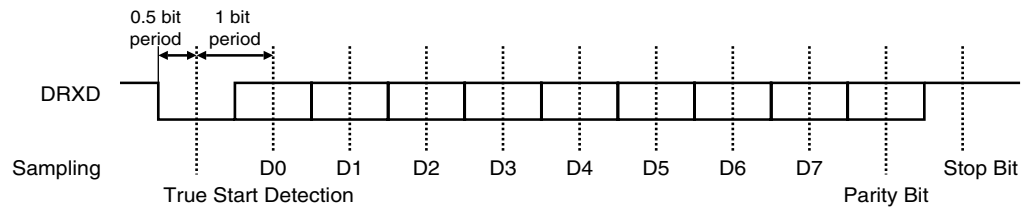
Figure 27-5. Character Reception
