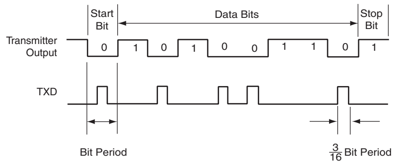
Figure 30-26. IrDA Modulation
