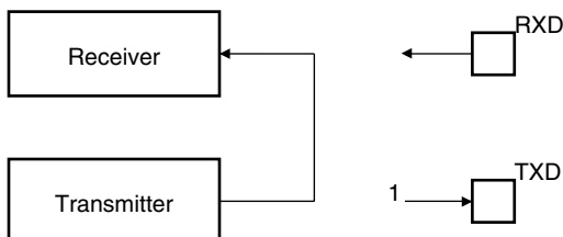
Figure 30-32. Local Loopback Mode Configuration
