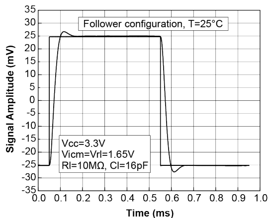
Figure 23. Small signal response at 3.3 V supply voltage
