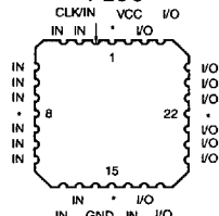
PLCC
