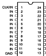
DIP/SOIC
