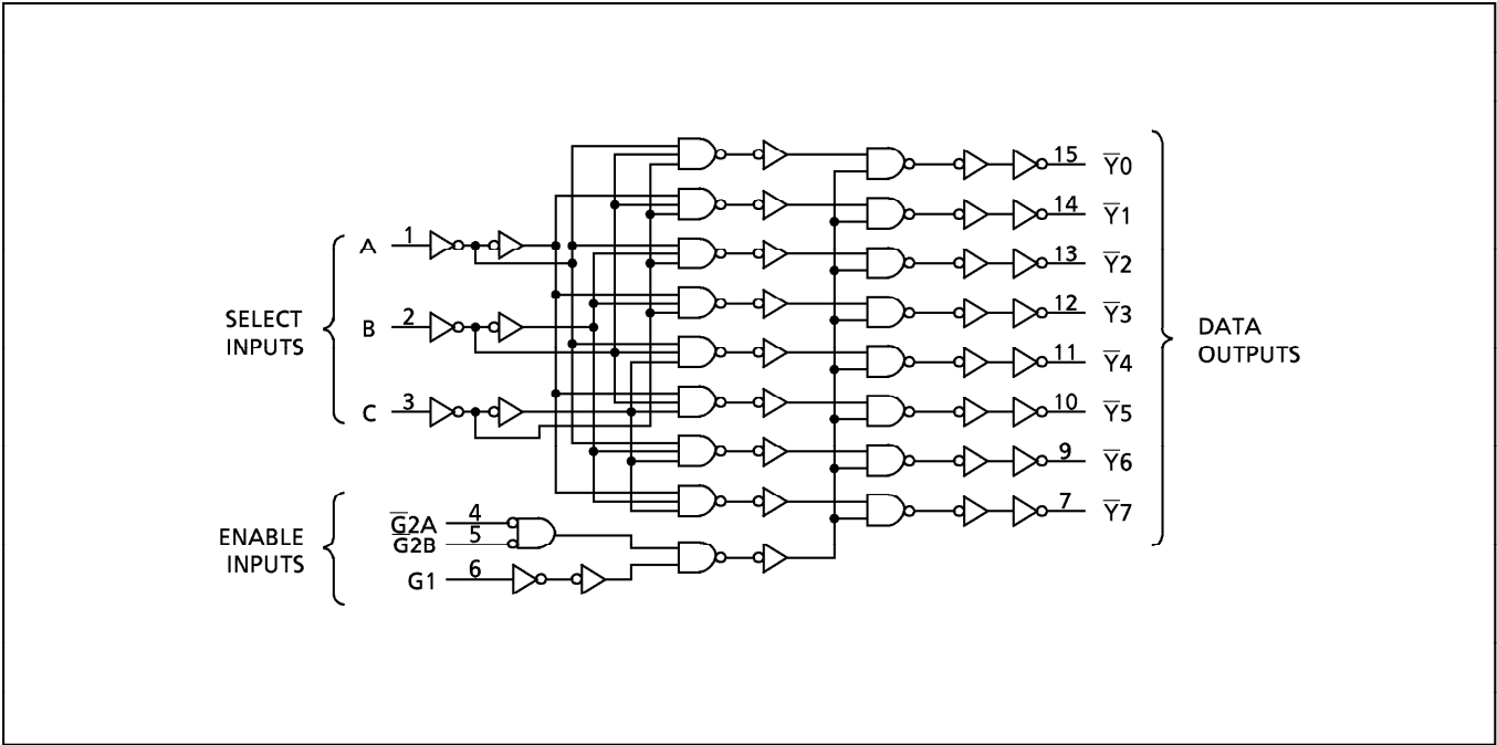
LOGIC DIAGRAM
