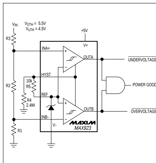
Figure 6. Window Detector
