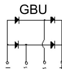
Case Style
